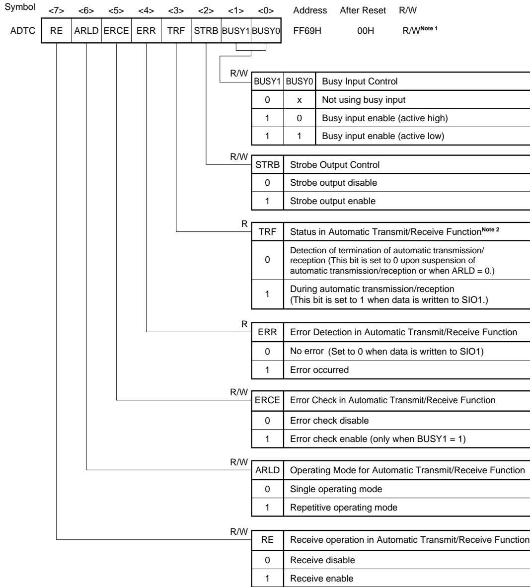
Figure 19-4. Automatic Data Transmit/Receive Control Register Format
