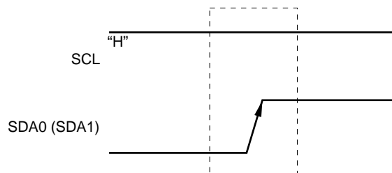
Figure 18-19. Stop Condition
