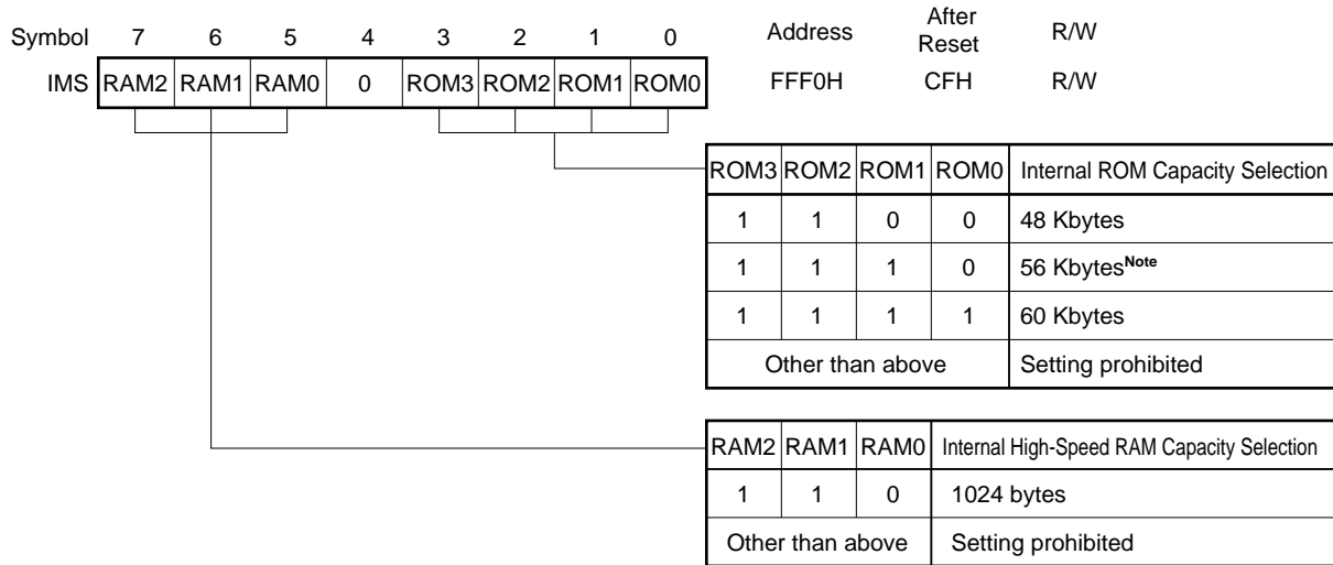
Figure 27-1. Internal Memory Size Switching Register Format
