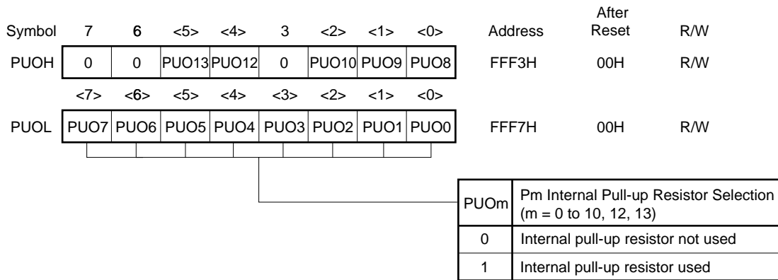
Figure 6-25. Pull-Up Resistor Option Register Format
