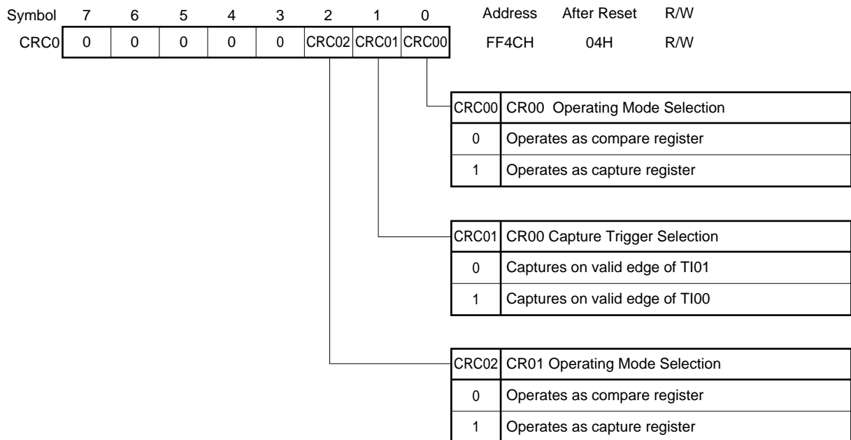
Figure 8-5. Capture/Compare Control Register 0 Format
