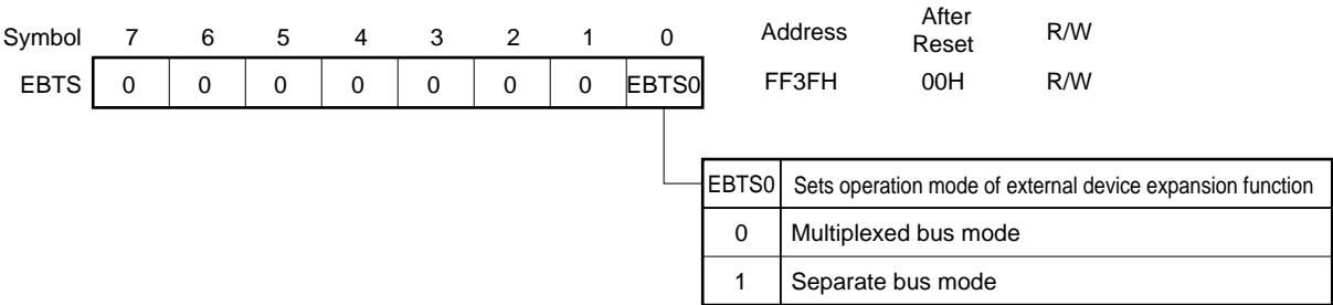
Figure 23-4. External Bus Type Select Register Format
