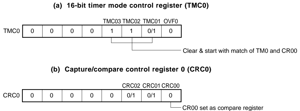
Figure 8-26. Control Register Settings in External Event Counter Mode
