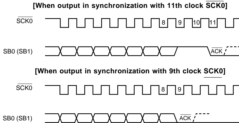
Figure 17-18. Acknowledge Signal
