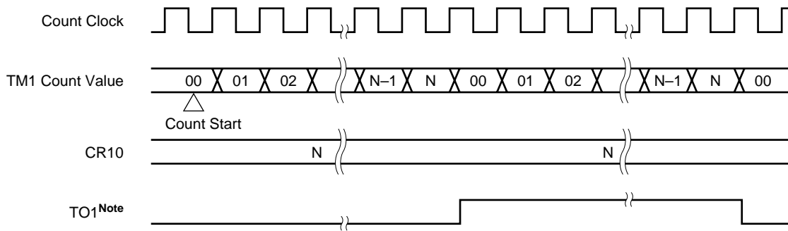
Figure 9-10. Timing of Square Wave Output Operation
