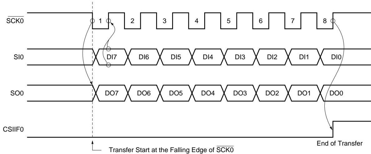
Figure 17-7. 3-Wire Serial I/O Mode Timings
