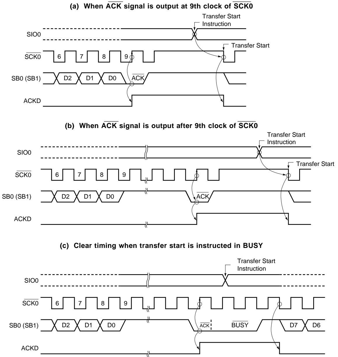
Figure 17-25. BSYE Operation
