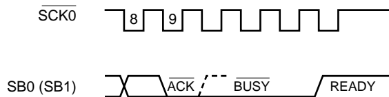
Figure 17-19. \overline{\text{BUSY}} and READY Signals
