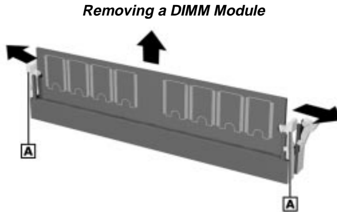
A – Plastic Clips
