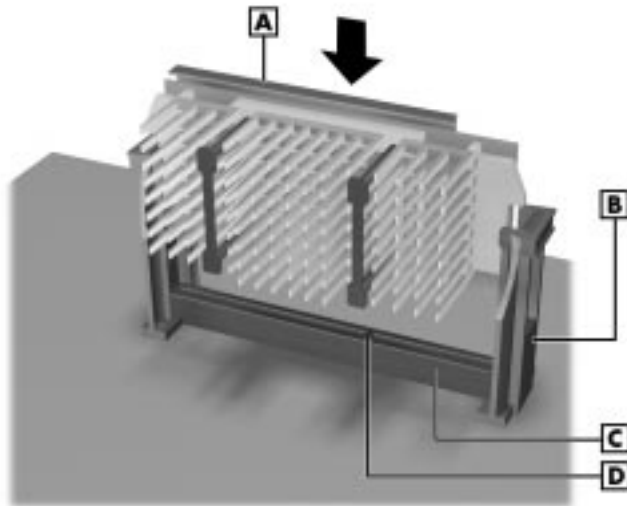
A – Processor Cartridge C – Slot 1 Connector B – Retention Mechanism D – Key
