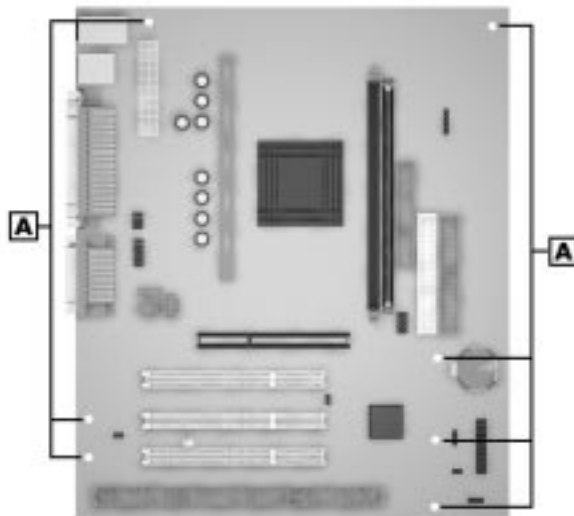
A – Screws
