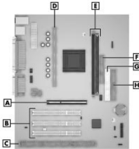
System Board Internal Connector and Socket Locations
