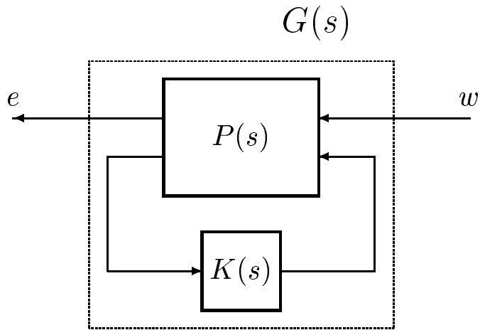
Figure 2.8: Closed loop system, G(s) , for performance analysis
