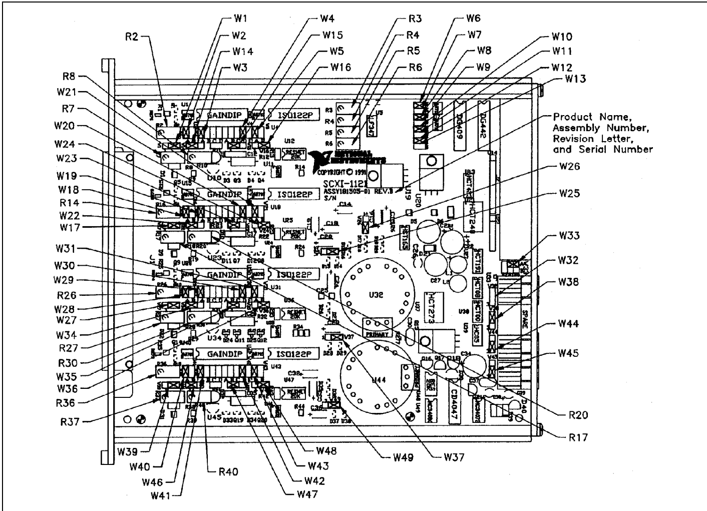
Figure F-3. Revision A and B SCXI-1121 Detailed Parts Locator Diagram
