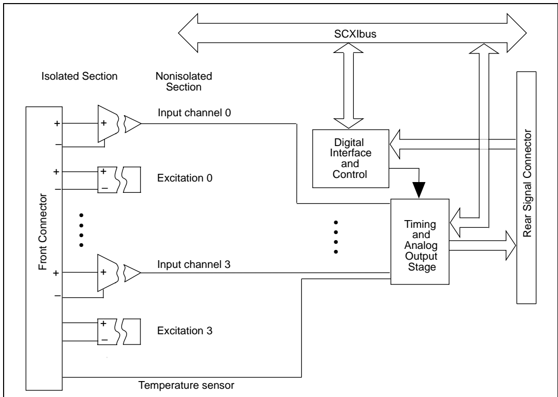
Figure 3-1. SCXI-1121 Block Diagram
