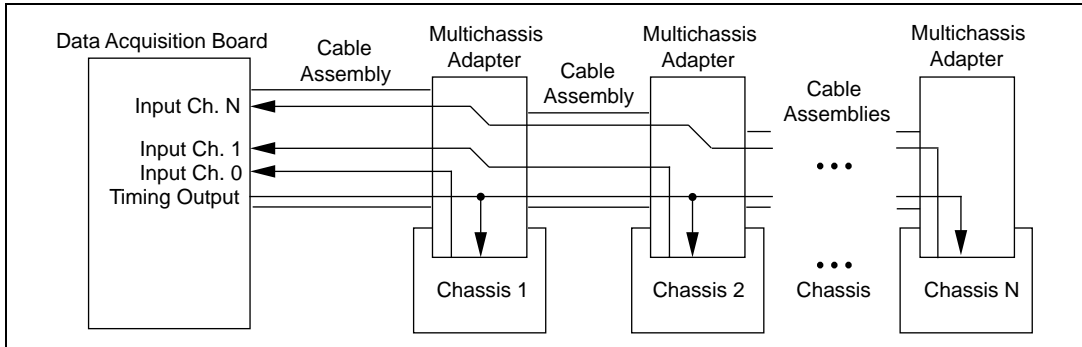
Figure 3-11. Multiple-Chassis Scanning
