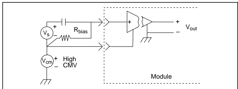
Figure 2-7. AC-Coupled Signal Connection with High Common-Mode Voltage
