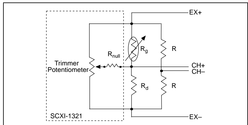
Figure 2-9. Nulling Circuit
