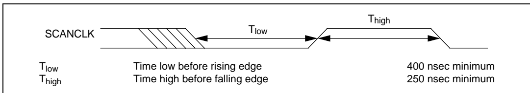
Figure 2-15. SCANCLK Timing Requirements
