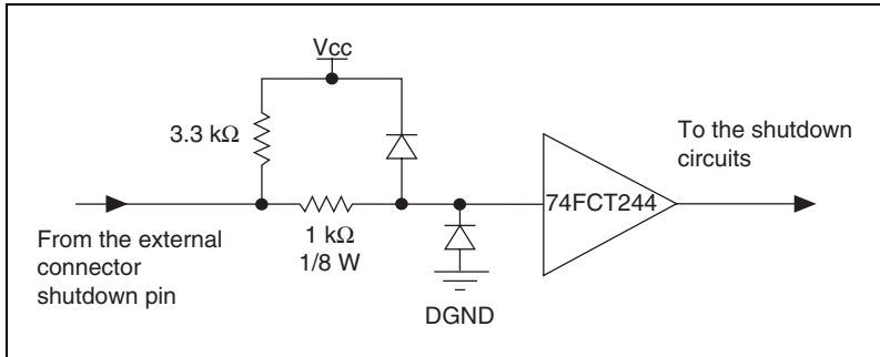
Figure 5-6. Shutdown Input Circuit
