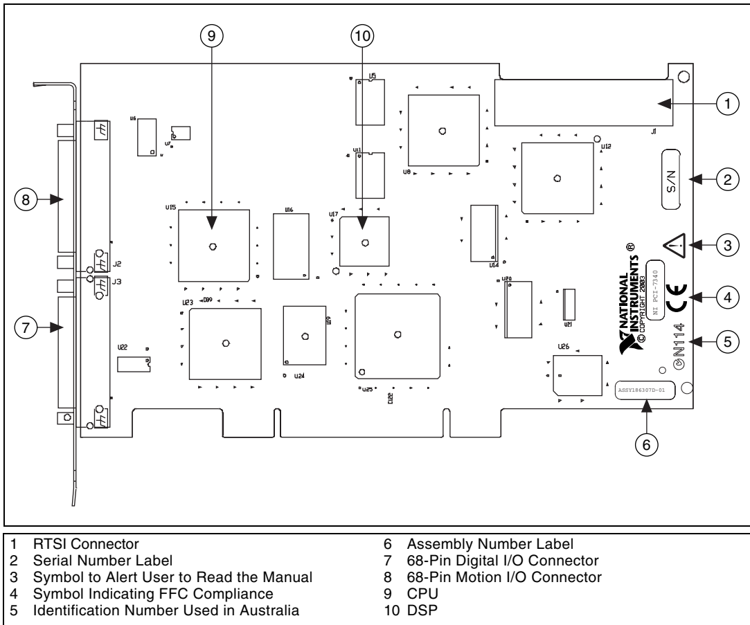
Figure 3-3. PCI-7340 Parts Locator Diagram
