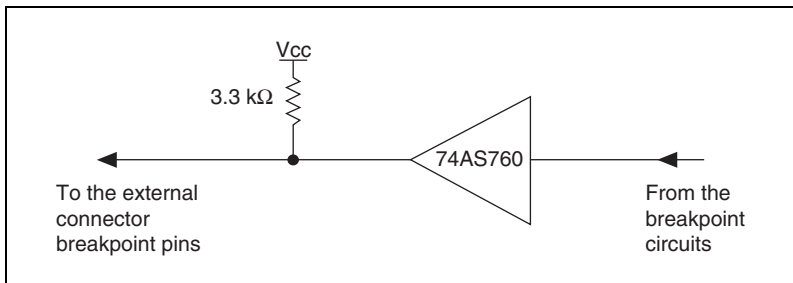
Figure 5-7. Breakpoint Output Circuit
