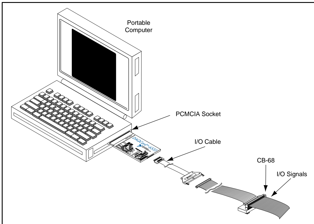
Figure 2-1. DAQCard-6533 Completed Installation
