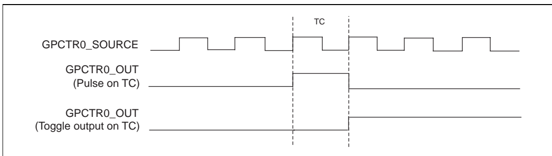
Figure 4-10. GPCTR0_OUT Signal Timing
