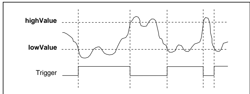
Figure 3-7. Low-Hysteresis Triggering Mode
