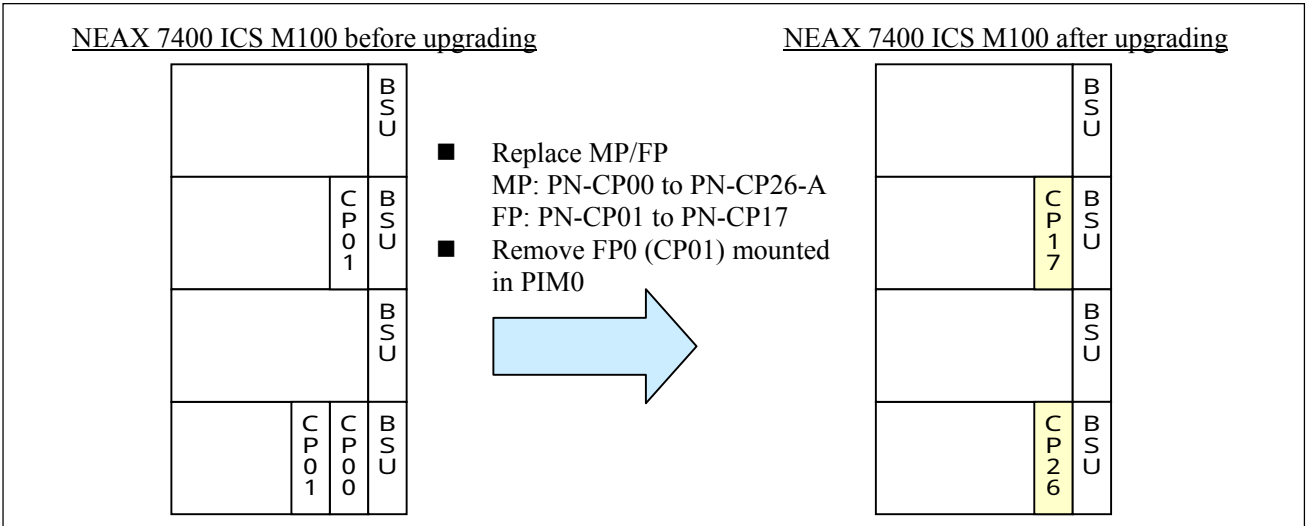
Figure 1-4 Retrofit MP/FP for Upgrading NEAX 7400 ICS M100 to IPS (Single MP System)
