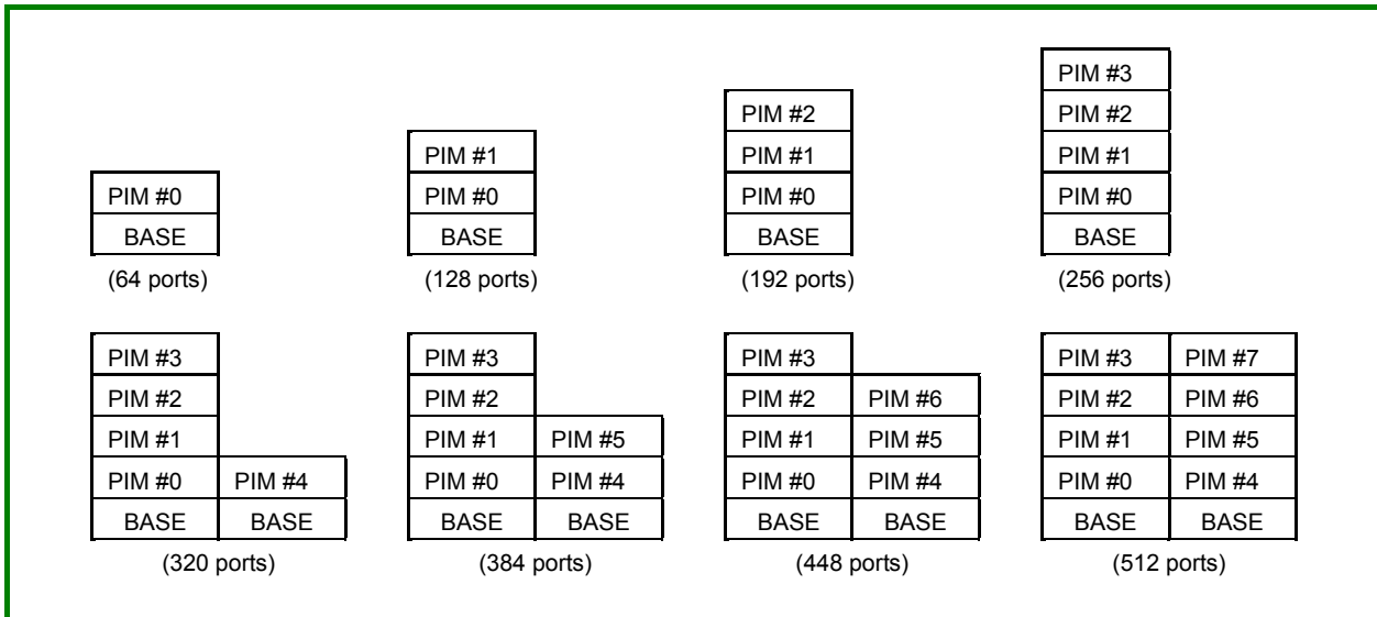
Figure 2-2 Face Layout of NEAX 2000 IPS
