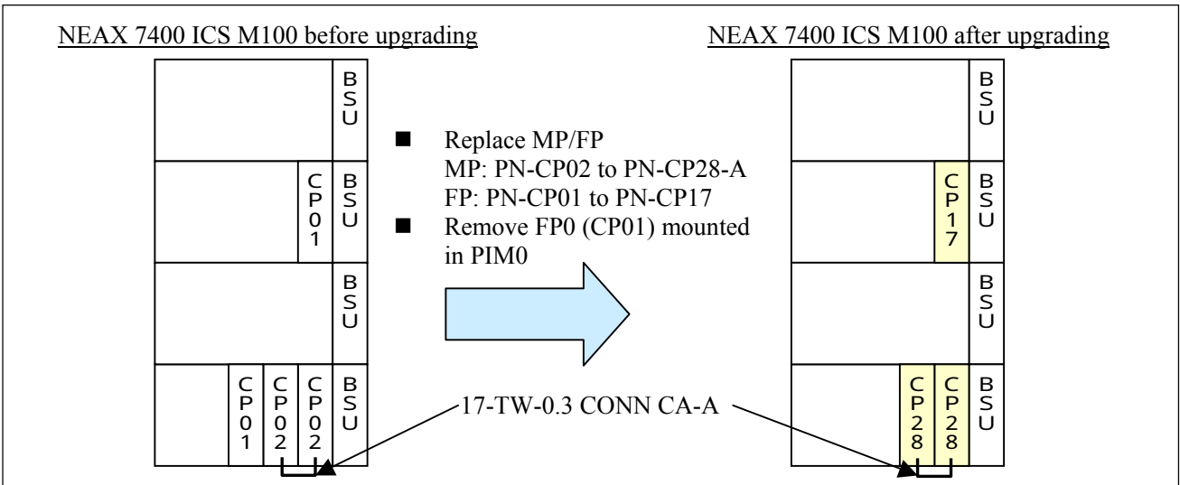
Figure 1-5 Retrofit MP/FP for Upgrading NEAX 7400 ICS M100 to IPS (Dual MP System)
