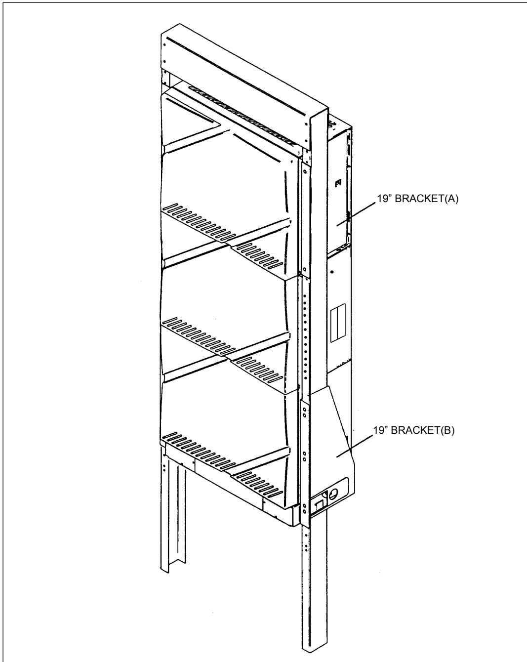
Figure 2-4 19-inch Rack-mounting
