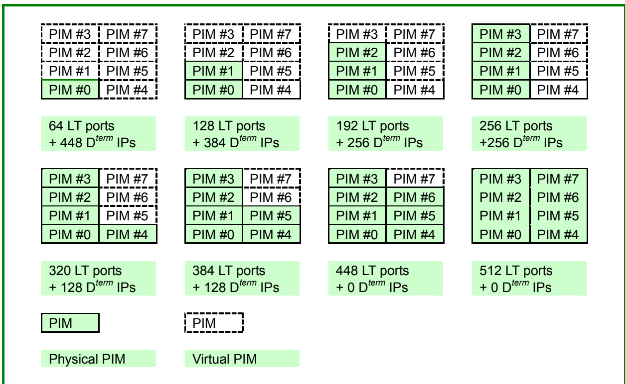
Figure 2-1 Module Configuration of NEAX 2000 IPS
