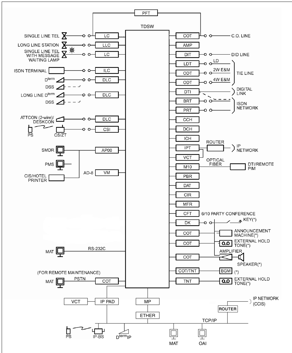
Figure 1-6 Trunking Diagram of NEAX 2000 IPS
