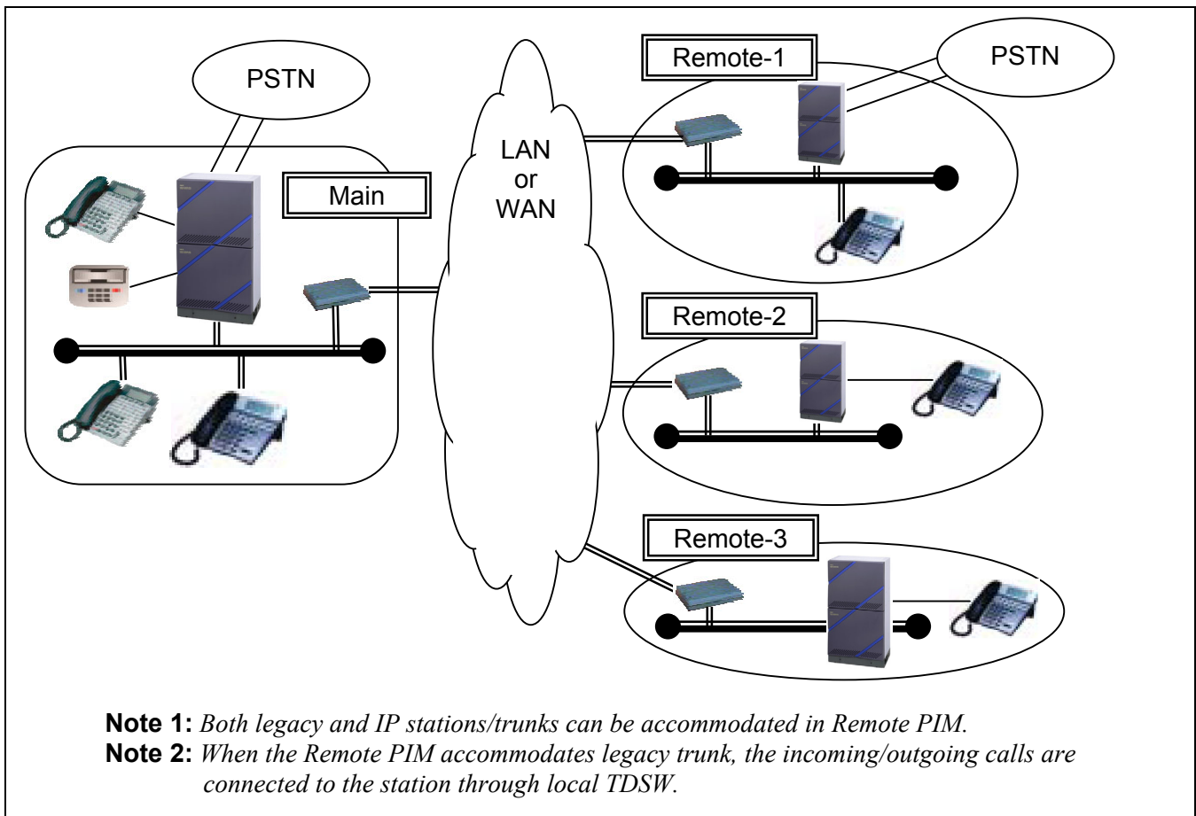
Figure 1-3 Example of Network Configuration of Remote PIM over IP
