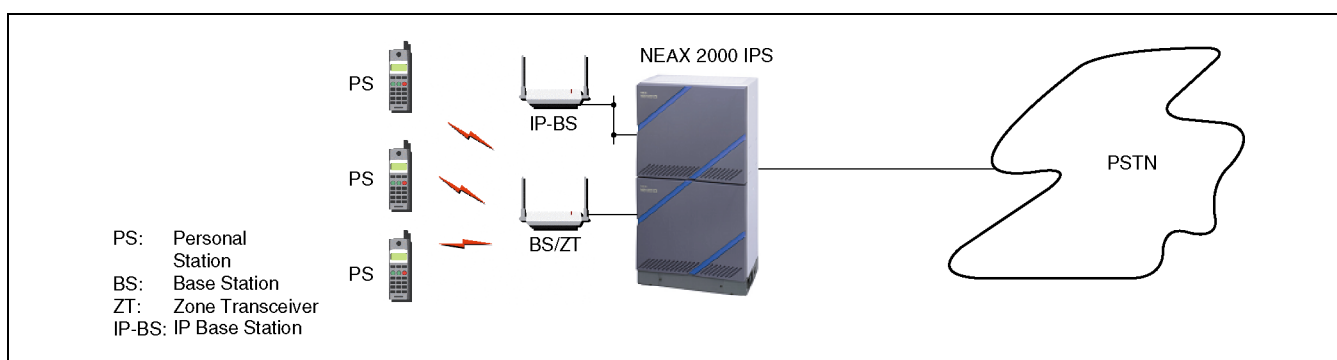
Figure 3-13 System Configuration of Wireless Communications
