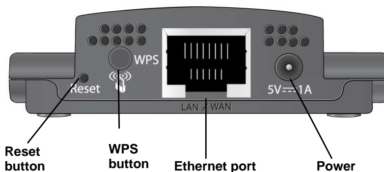
Figure 1. Rear panel
