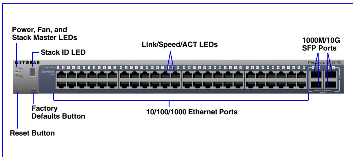
Figure 2. Front Panel
