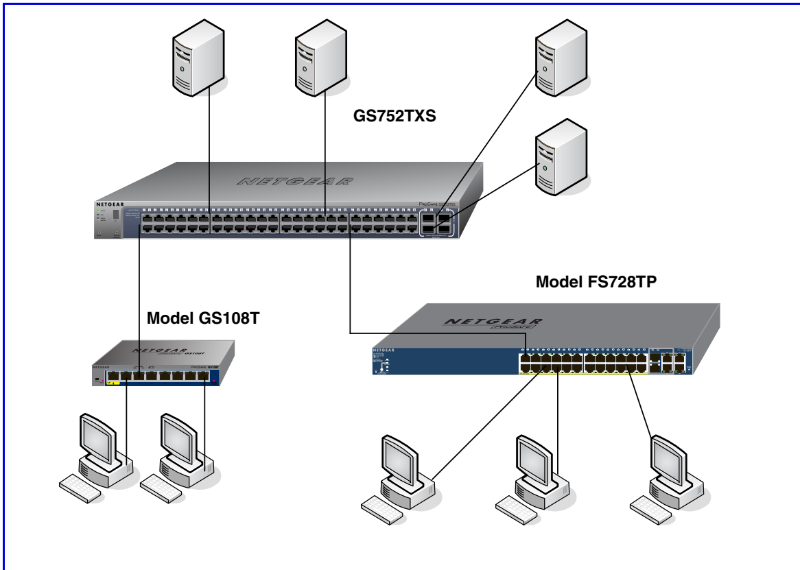
Figure 5. Backbone Switching
