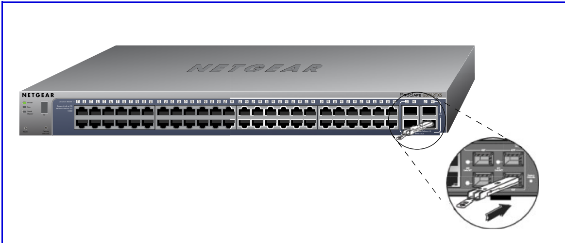
Figure 8. Installing and SFP Transceiver Module
