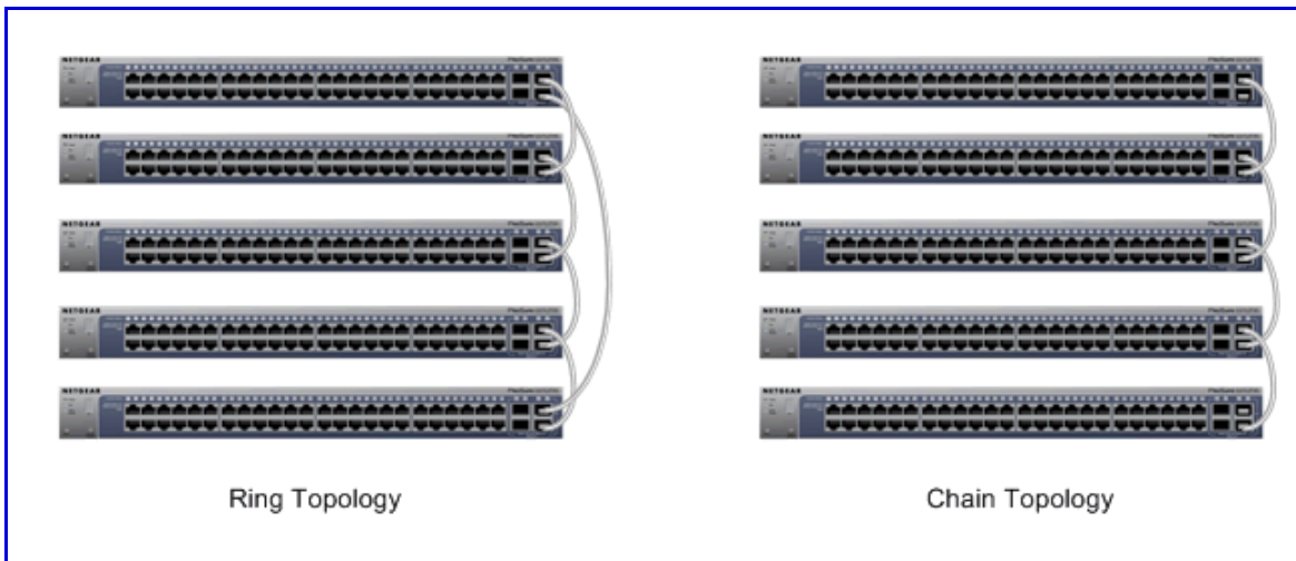
Figure 9. Stacking Topologies
