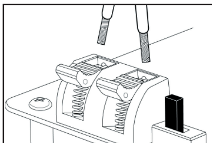
Figure 15. Connecting a loudspeaker wire to the HDFX terminals.
