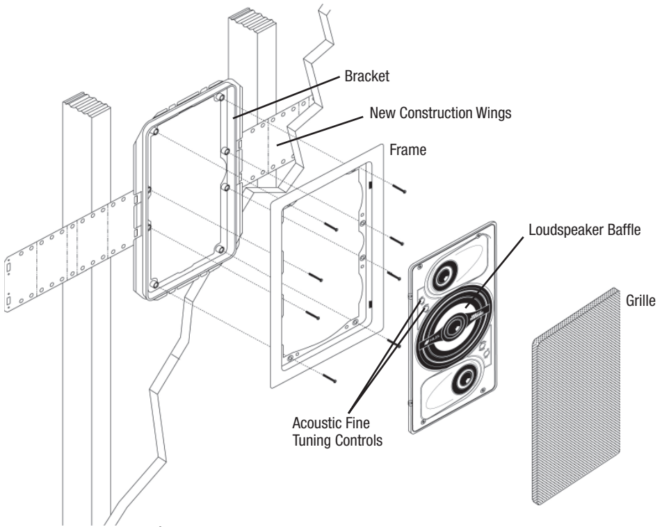
Figure 1. Mounting an HDFX vertically into a wall
