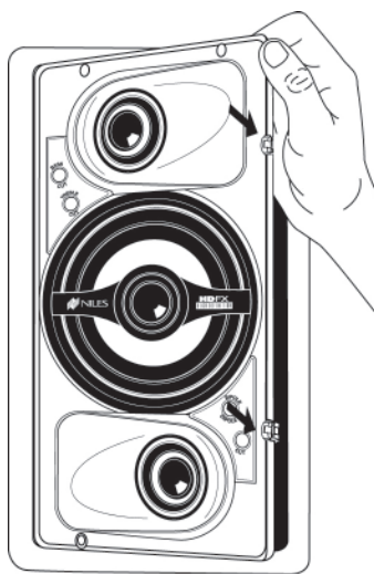
Figure 16. Installing the loudspeaker baffle into its frame.
