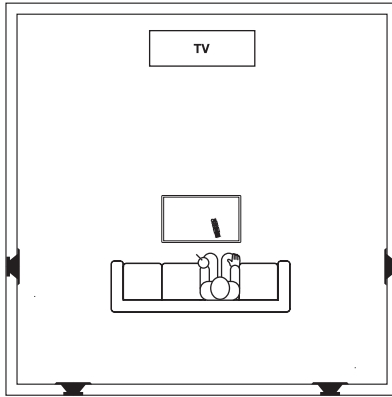
Figure 4. Two pairs of HDFX loudspeakers reproduce Dolby EX surround sound in a home theater room.
