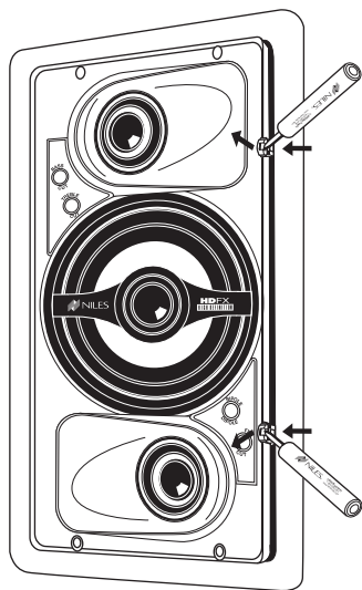
Figure 20. Removing the HDFX loudspeaker baffle from its frame.
