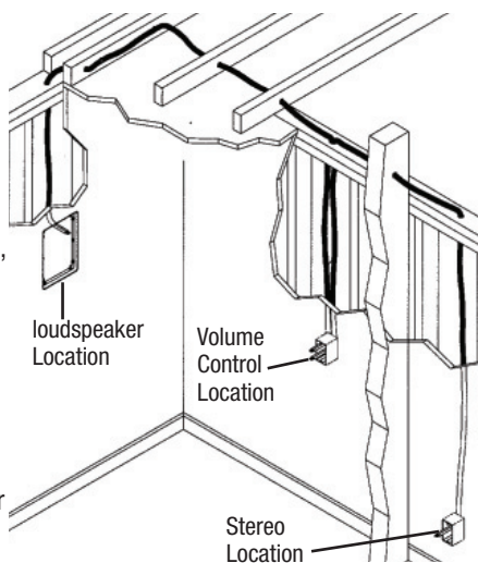
Figure 6. Running loudspeaker wire from a wall loudspeaker to a home theater system location.
