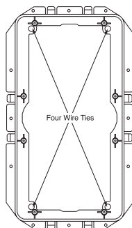
Figure 11. The brackets have four wire-tie points.
