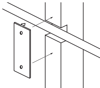
Figure 5. Installing a nail plate to protect wiring in a notched stud.
