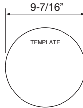
Cutout template x1
