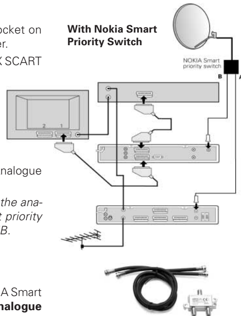
Nokia Smart Priority Switch
