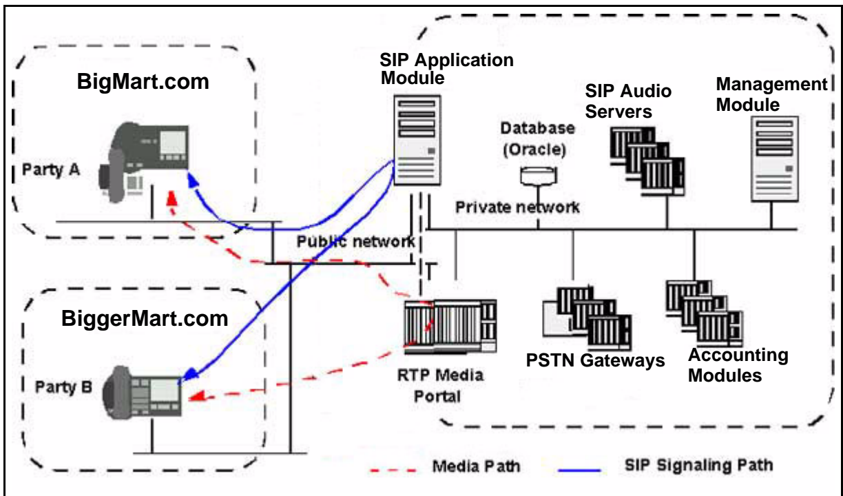
Figure 2 Example of network configuration
