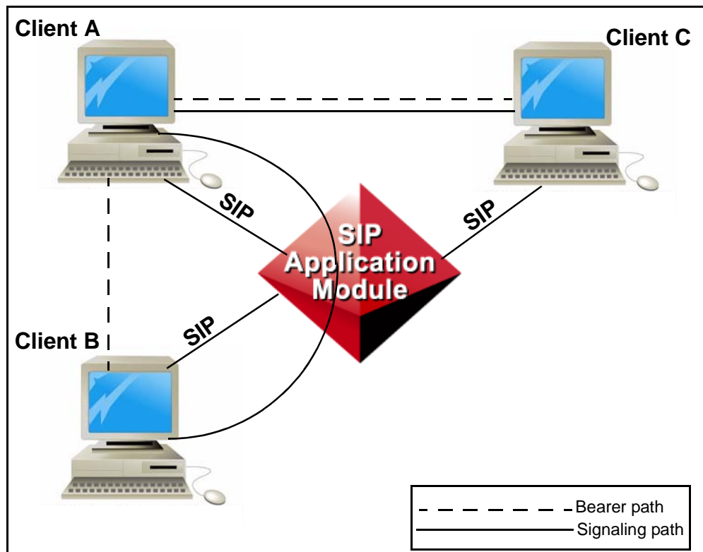
Figure 3 Call transfer to client diagram
