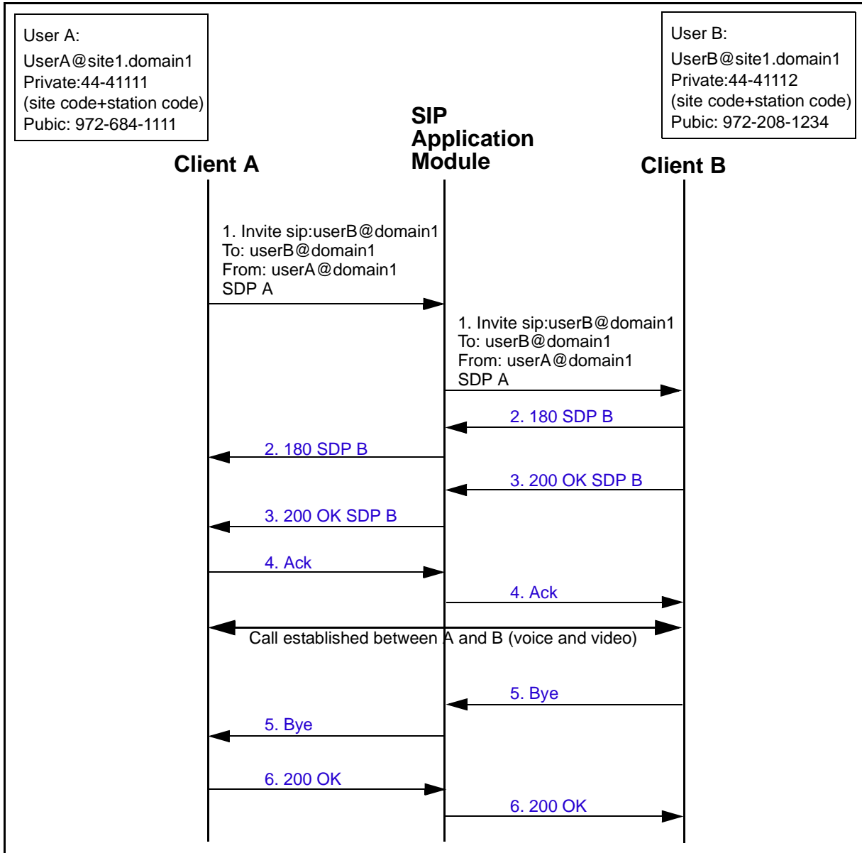
Figure 2 Client-to-client voice plus video call flow
