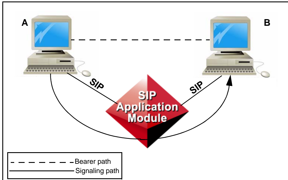
Figure 1 Client-to-client voice plus video diagram
