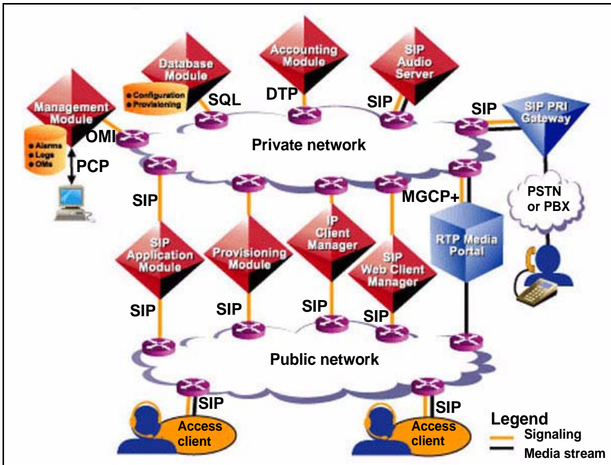
Figure 4 Protocols
