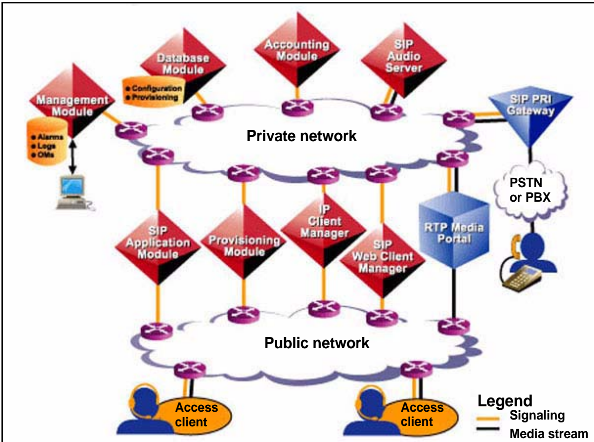
Figure 3 Network interfaces
