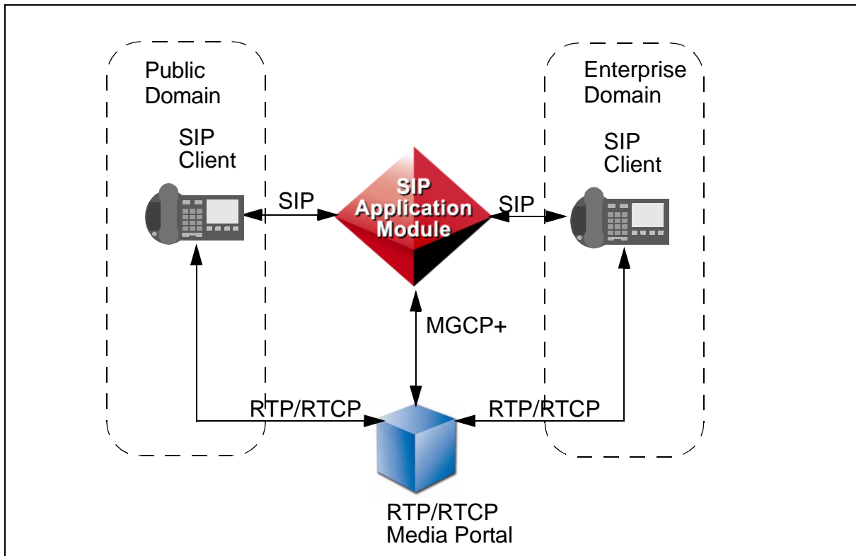
Figure 6 RTP Media Portal interworking with Enterprise or foreign clients
