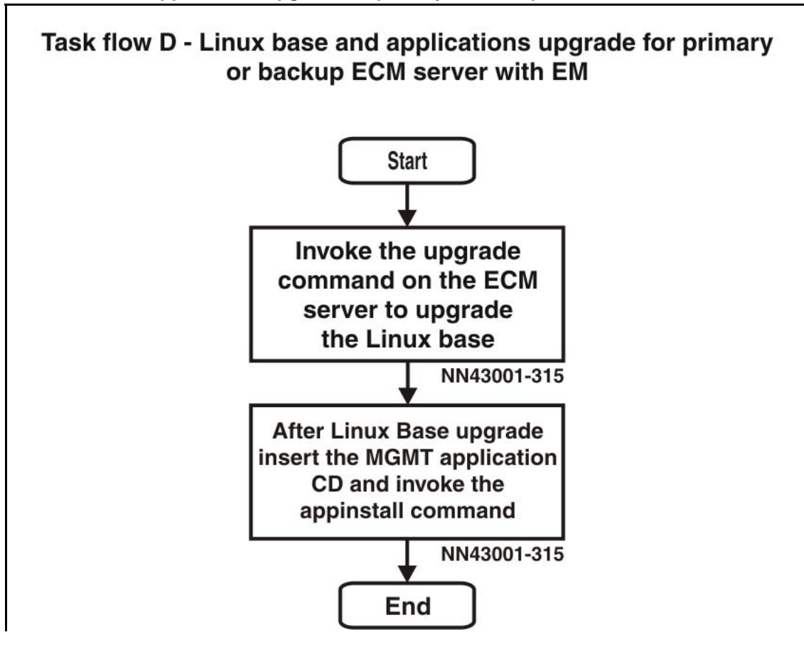
Figure 4 Linux base and applications upgrade for primary or backup ECM server with EM
