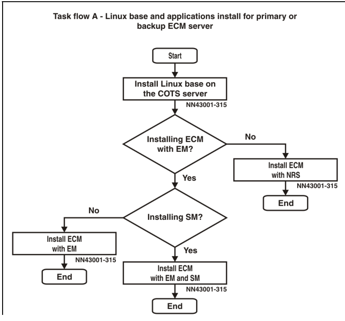
Figure 1 Linux base and applications install for primary or backup ECM server
