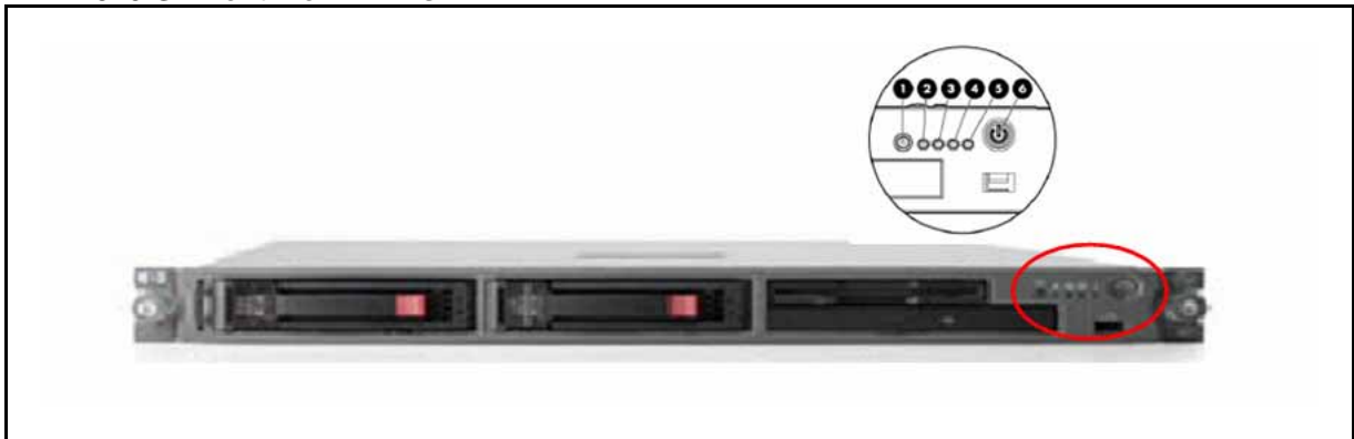
Figure 113 HP DL320 G4 front view: LEDs
