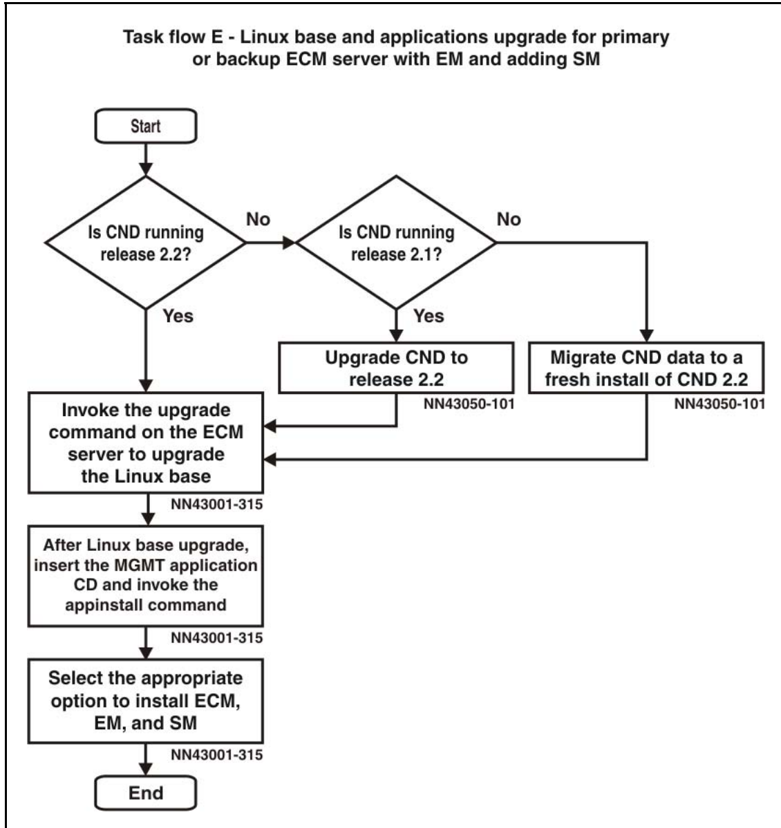
Figure 5 Linux base and applications upgrade for primary or backup ECM server with EM and adding SM
