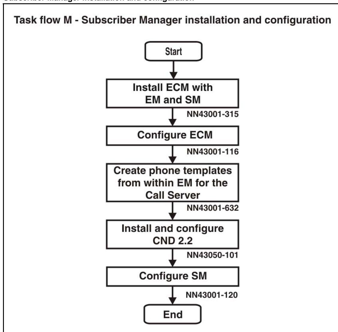
Figure 13 Subscriber Manager installation and configuration
