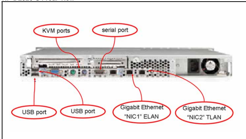
Figure 114 HP DL320 G4 rear view
