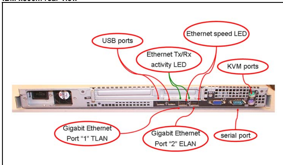
Figure 123 IBM x306m rear view
