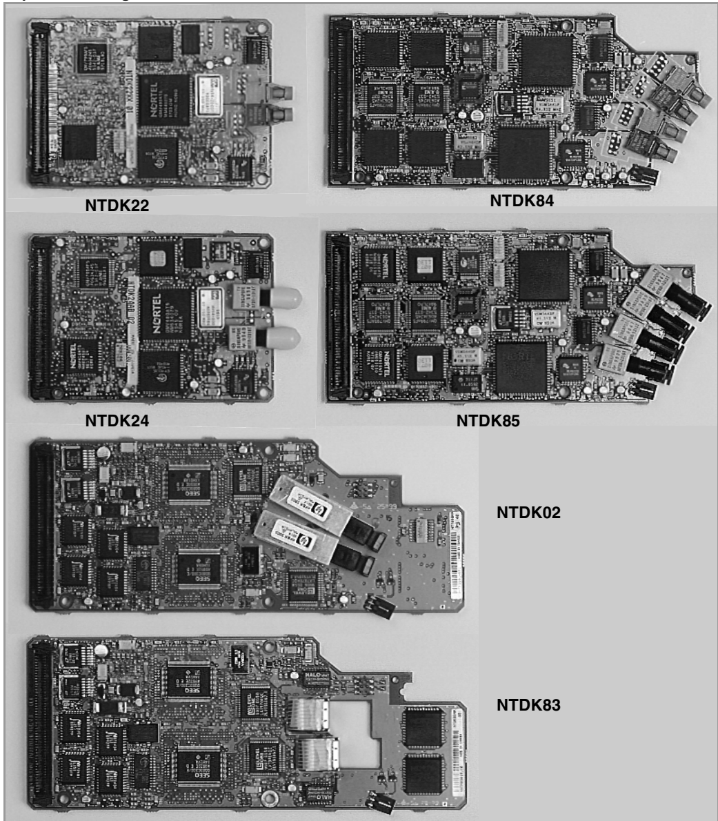
Figure 19 Expansion Daughterboards
