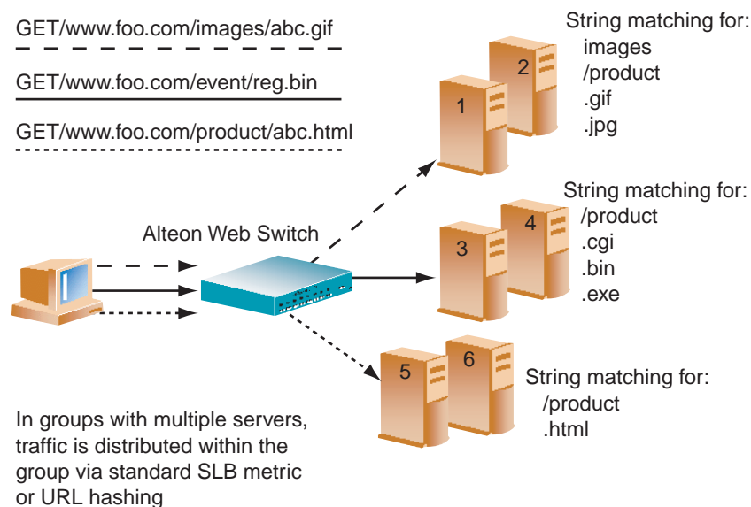
Figure 15-2 URL-Based Server Load Balancing
