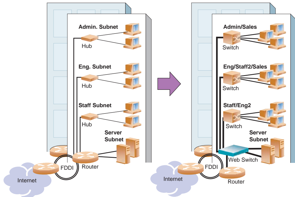
Figure 1-1 The Router Legacy Network
