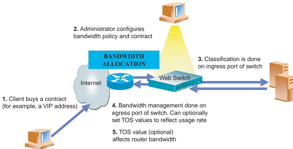
Figure 17-1 Bandwidth Management: How It Works
