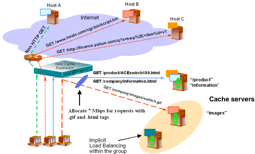
Figure 17-5 URL-Based Bandwidth Management with Web Cache Redirection
