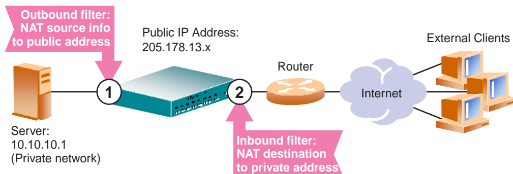
Figure 7-8 Static Network Address Translation
