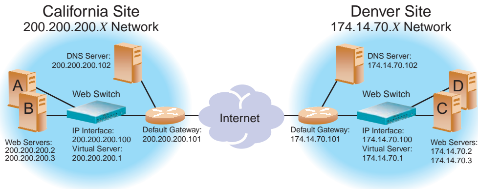
Figure 12-2 GSLB Topology Example
