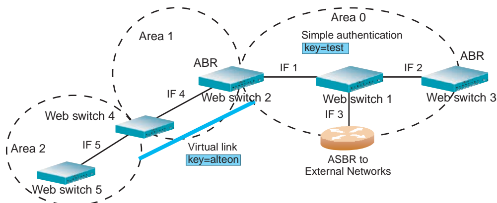
Figure 4-4 OSPF Authentication
