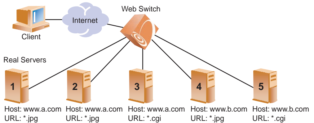
Figure 15-8 Content Precedence Lookup Multiple Strings Example
