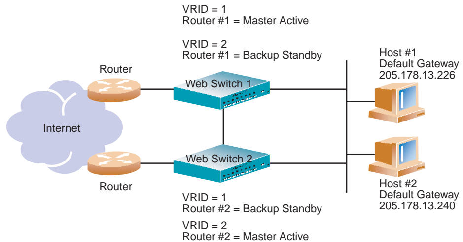
Figure 11-2 Example 2: VRRP Router
