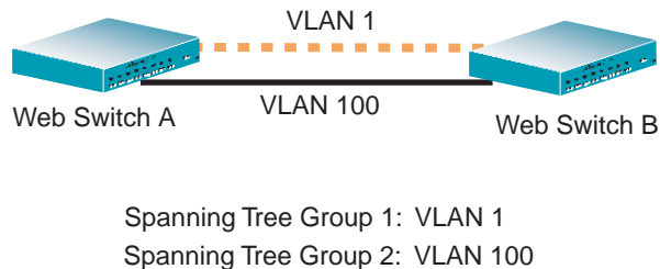
Figure 2-3 Using Multiple Instances of Spanning Tree Protocol
