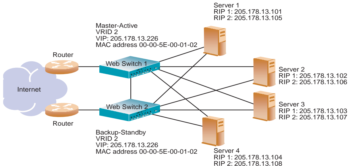
Figure 11-8 Active-Standby High-Availability Configuration
