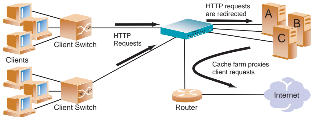
Figure 8-2 Network with Web Cache Redirection
