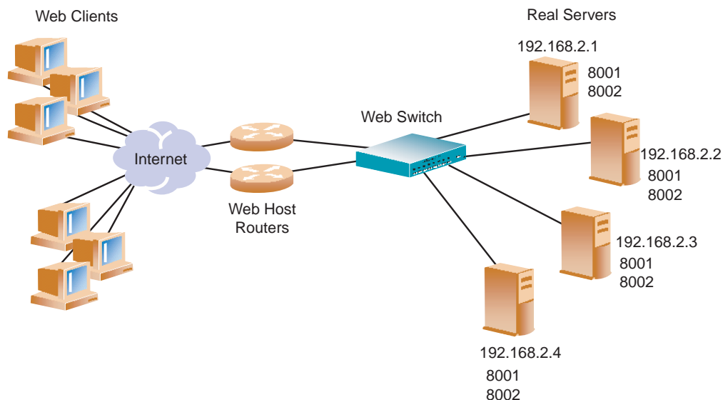
Figure 6-6 Basic Virtual Port to Real Port Mapping Configuration
