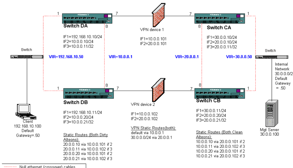
Figure 14-2 VPN Load-Balancing Configuration Example
