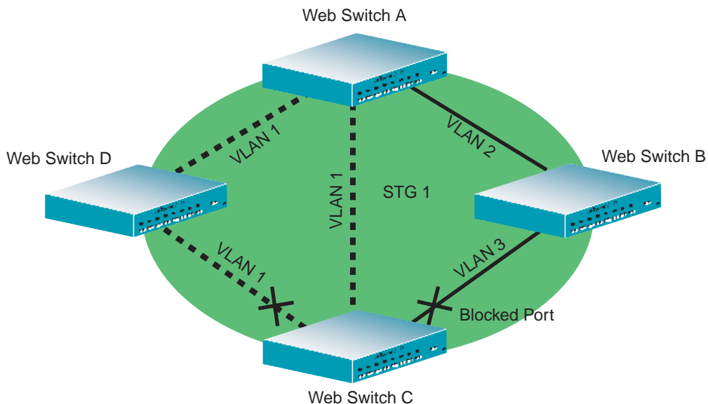
Figure 2-4 VLAN 3 Isolated in a Single Spanning Tree Group
