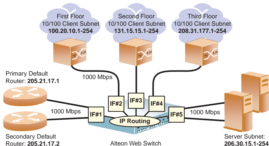
Figure 1-2 Switch-Based Routing Topology
