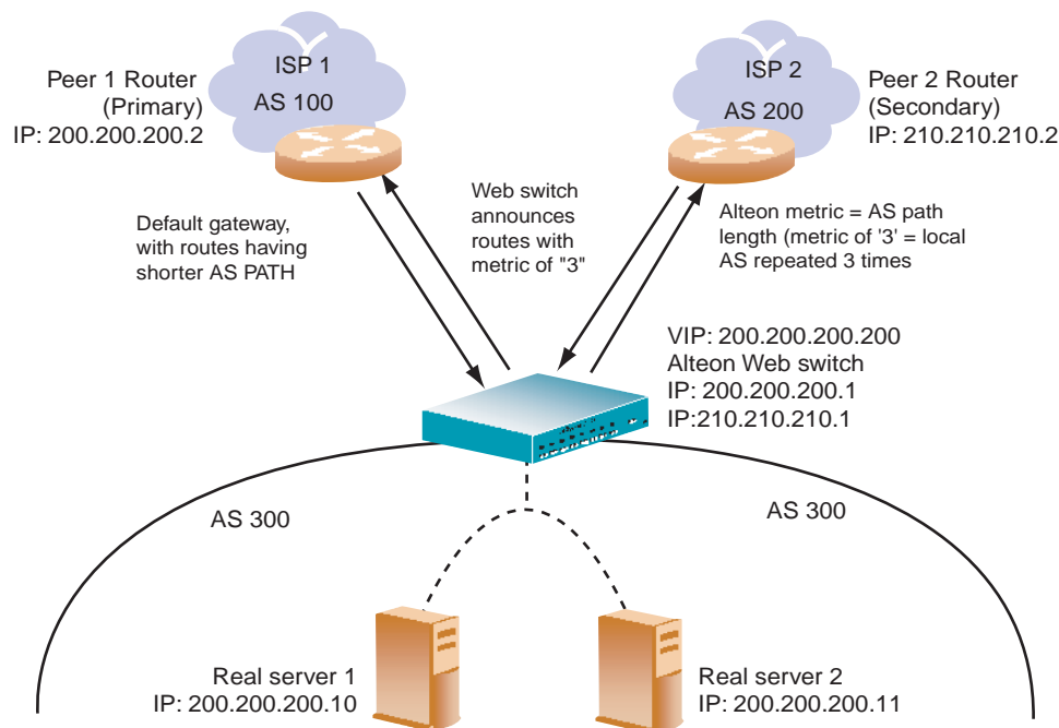
Figure 1-4 BGP Failover Configuration Example
