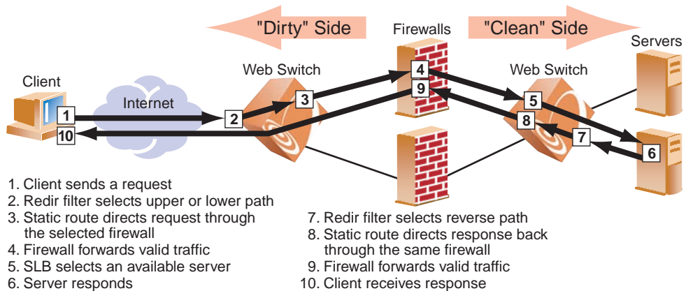
Figure 13-3 Basic FWLB Process
