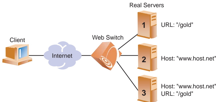
Figure 15-7 Content Precedence Lookup Protectors Example
