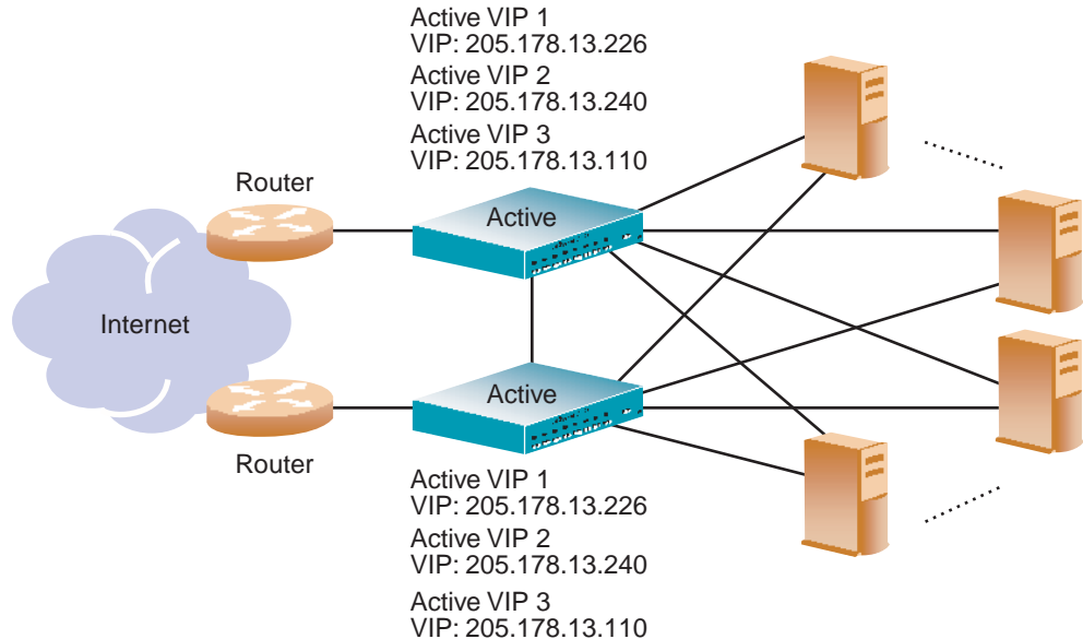
Figure 11-5 Active-Active Redundancy
