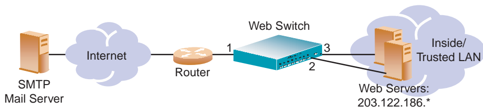
Figure 7-11 TCP ACK Matching Network
