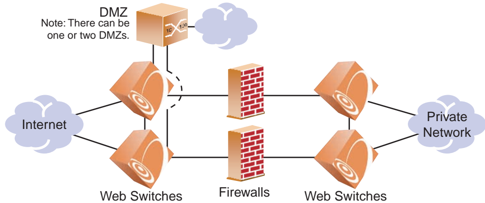
Figure 13-10 Typical Firewall Load-Balancing Topology with DMZ
