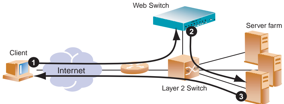
Figure 6-7 Direct Server Return
