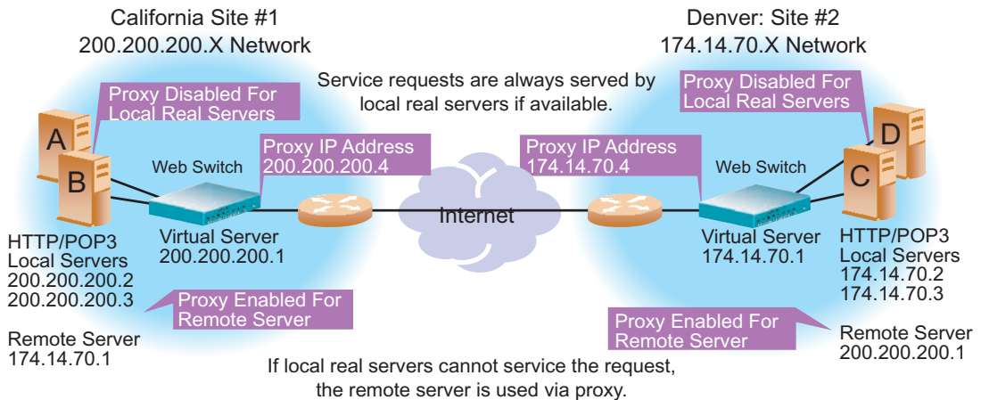
Figure 12-4 POP3 Request Fulfilled via IP Proxy
