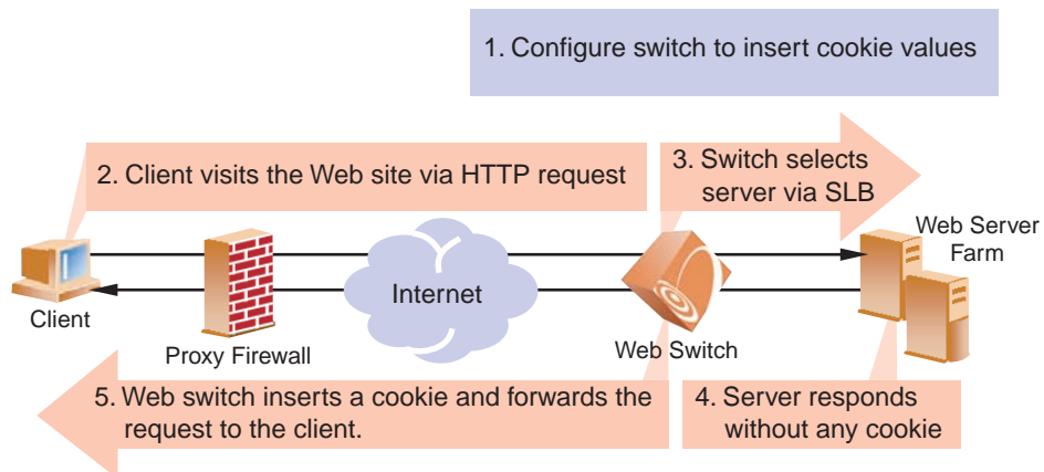
Figure 16-2 Insert Cookie Mode
