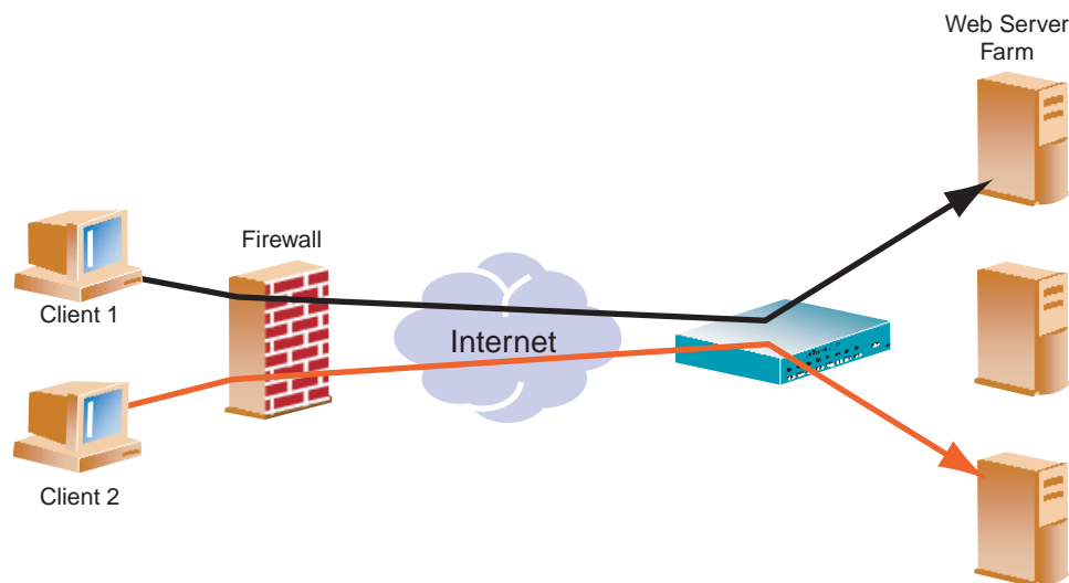
Figure 16-5 SSL Session ID-Based Persistence
