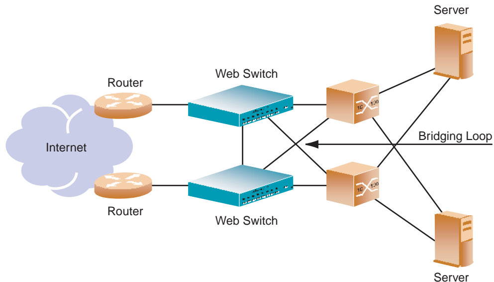
Figure 11-11 Loops in Active-Active Configuration
