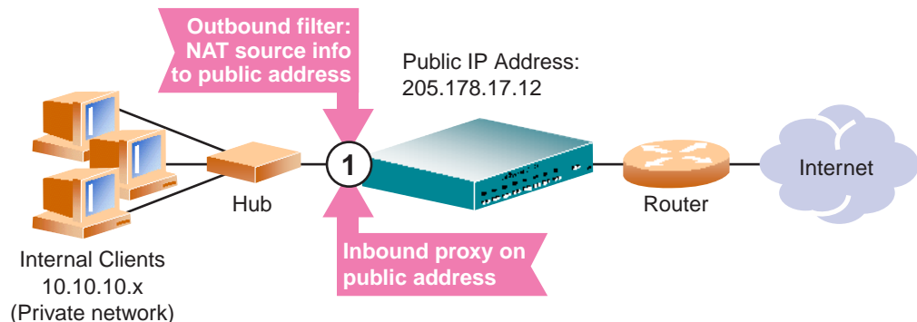
Figure 7-9 Dynamic Network Address Translation
