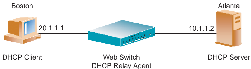
Figure 1-5 DHCP Relay Agent Configuration
