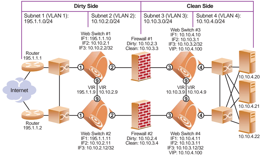
Figure 13-7 Four-Subnet FWLB Example Network
