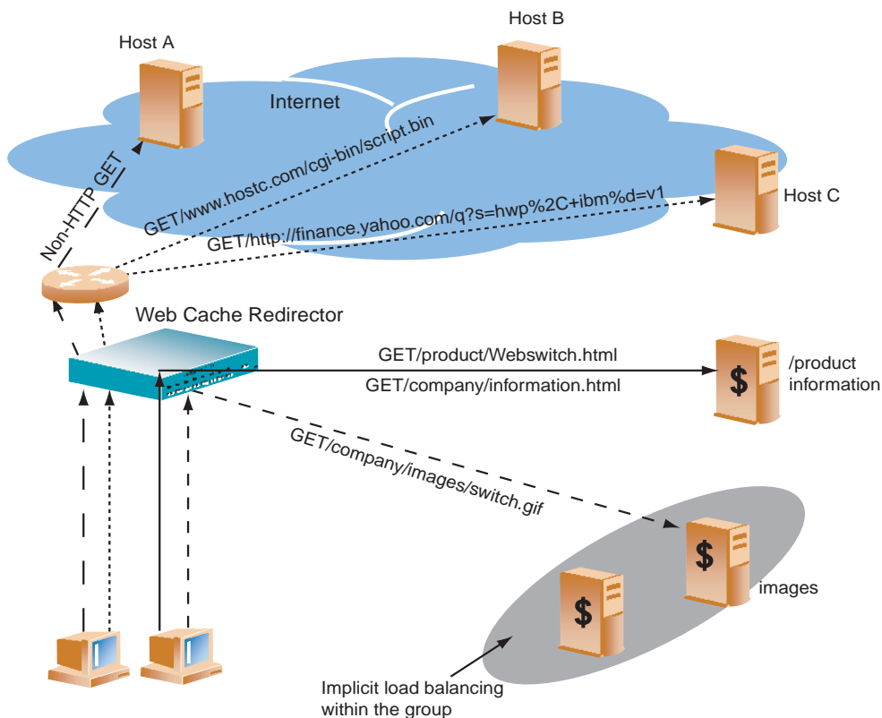
Figure 15-5 URL-Based Web Cache Redirection
