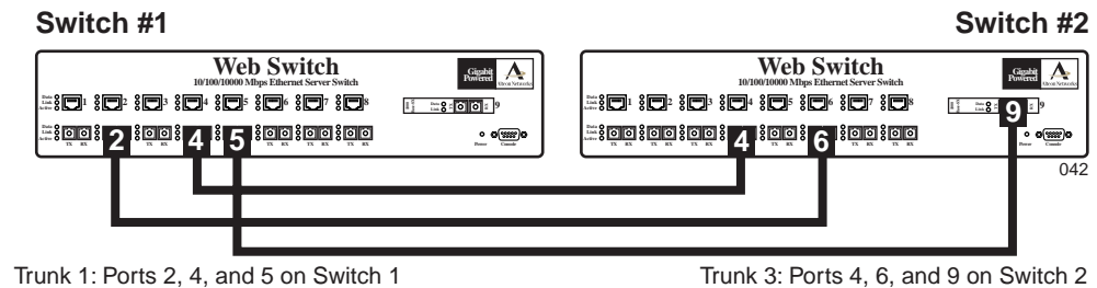
Figure 3-2 Port Trunk Group Configuration Example
