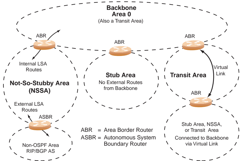
Figure 4-1 OSPF Area Types
