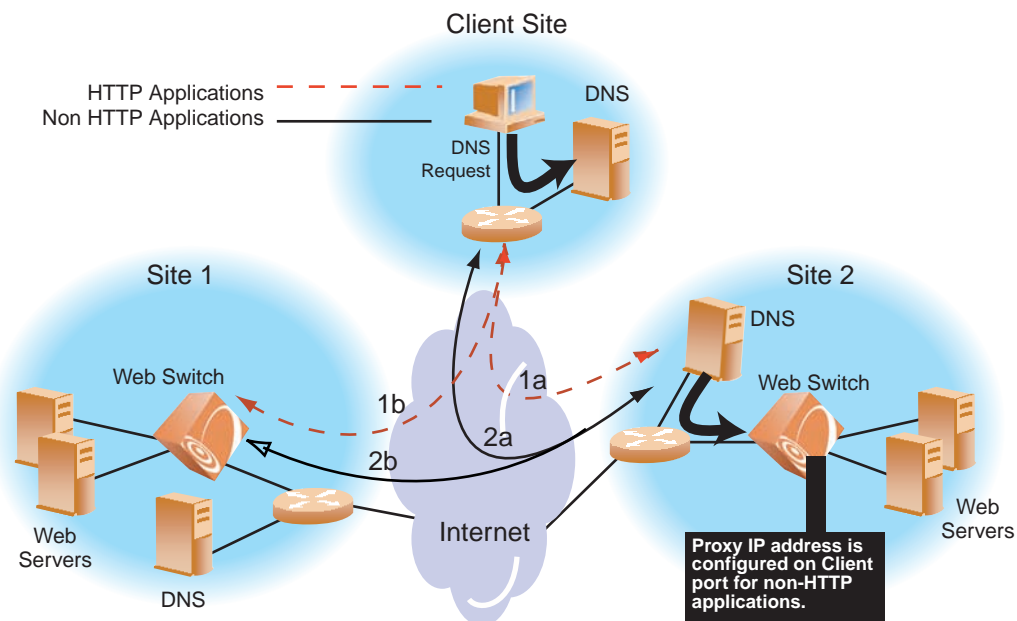
Figure 12-3 HTTP and Non-HTTP Redirects
