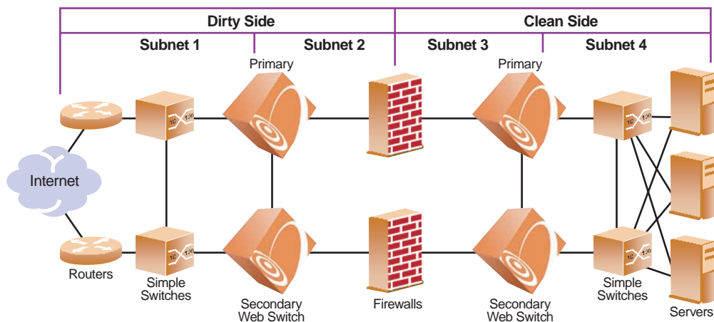
Figure 13-5 Four-Subnet FWLB Topology
