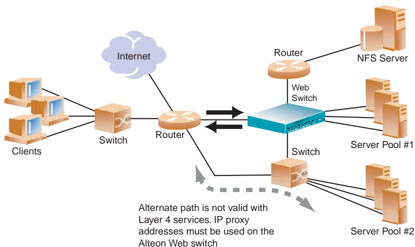
Figure 6-4 SLB Client/Server Traffic Routing
