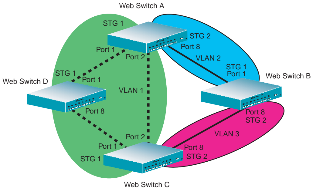
Figure 2-5 Implementing Multiple Spanning Tree Groups
