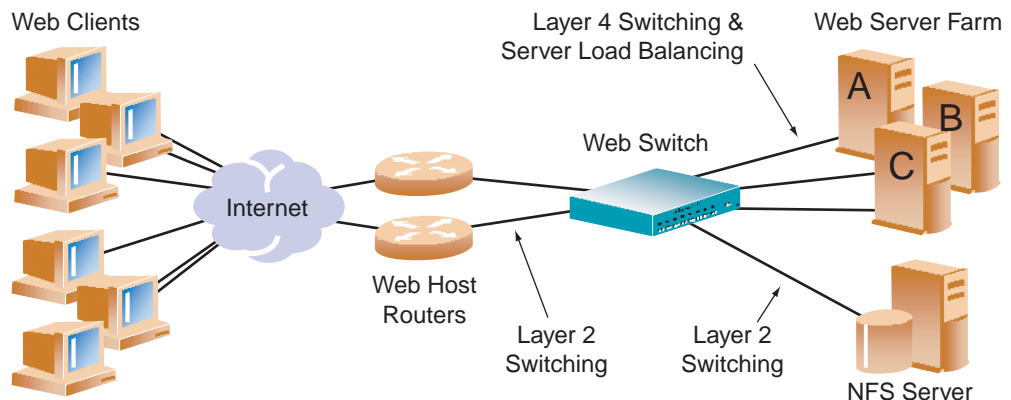
Figure 6-3 Web Hosting with SLB Solutions
