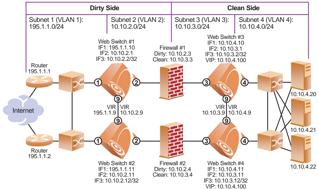
Figure 13-9 Four-Subnet FWLB Example Network
