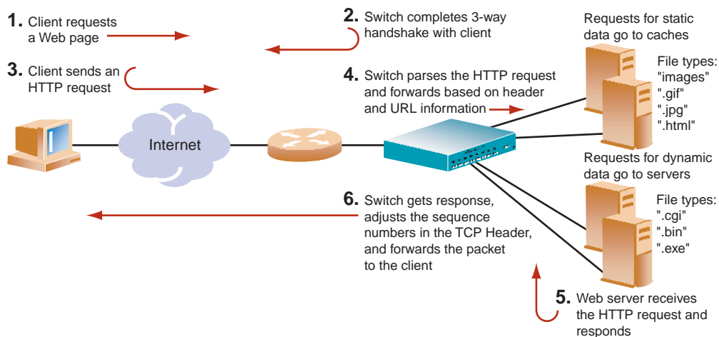
Figure 15-1 Content Intelligent Load Balancing Example
