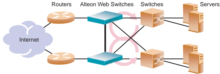
Figure 11-12 Cross-Redundancy Creates Loops, But STP Resolves Them
