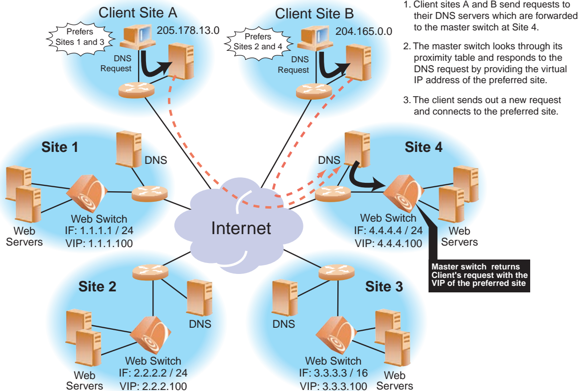
Figure 12-6 Configuring Client Proximity Table
