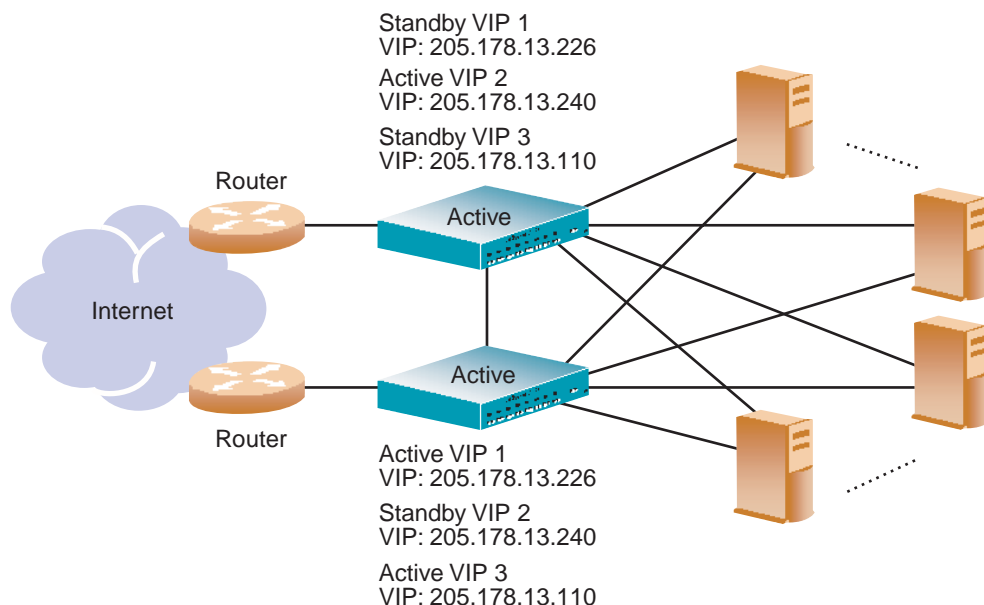
Figure 11-4 Active-Standby Redundancy
