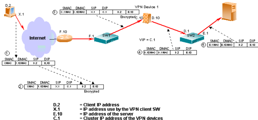
Figure 14-1 Basic Network Frame Flow and Operation
