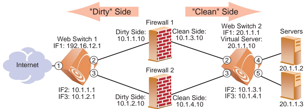
Figure 13-4 Basic FWLB Example Network
