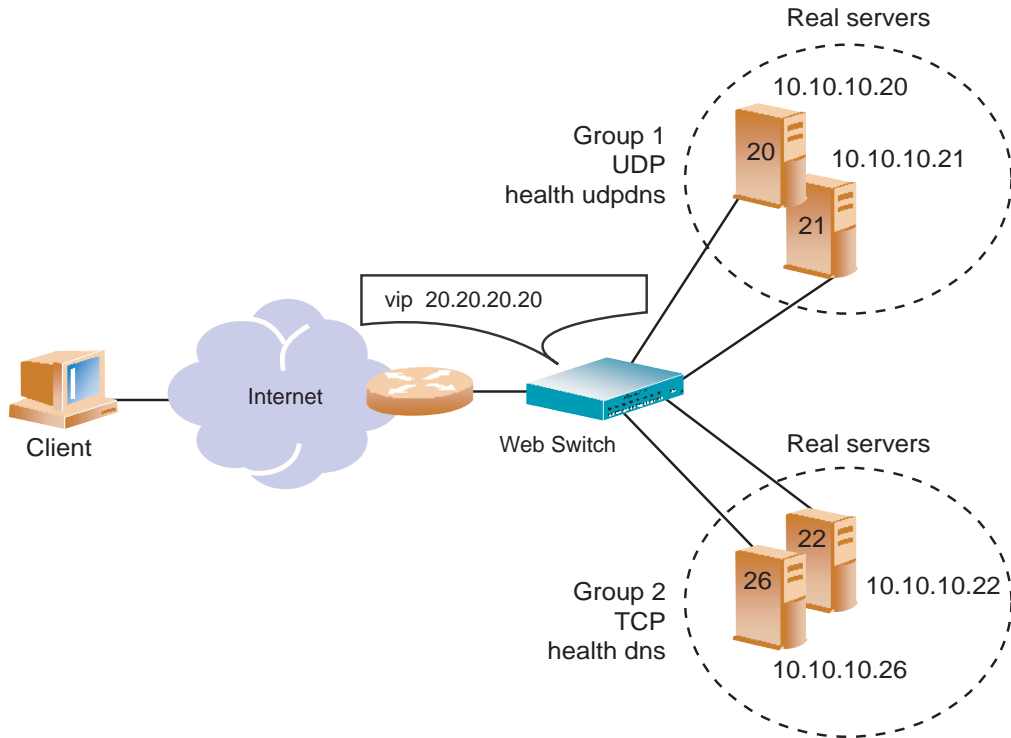
Figure 6-11 Layer 4 DNS Load Balancing
