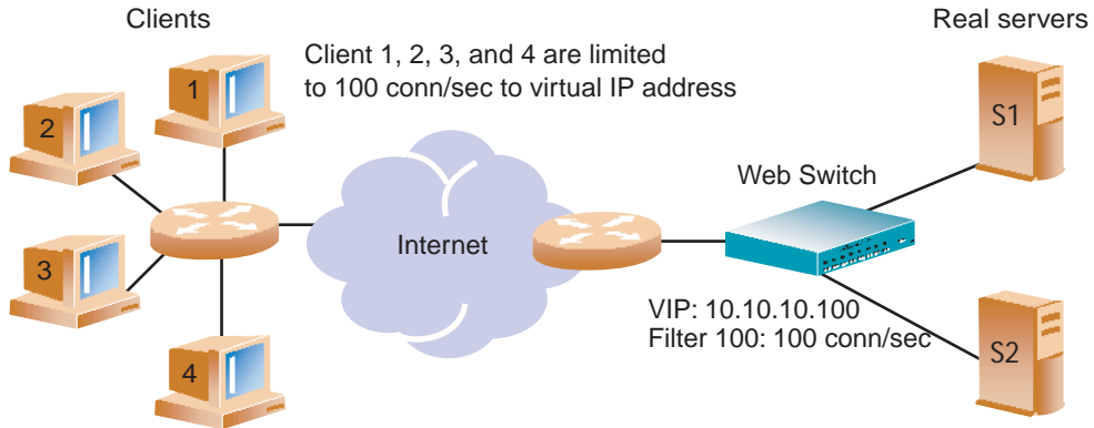
Figure 7-6 Limiting User Access to Server
