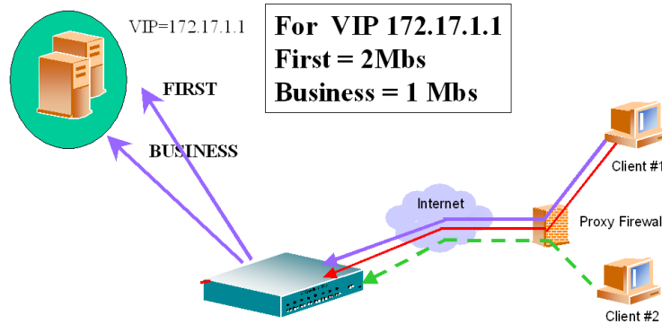
Figure 17-6 Cookie-Based Bandwidth Management
