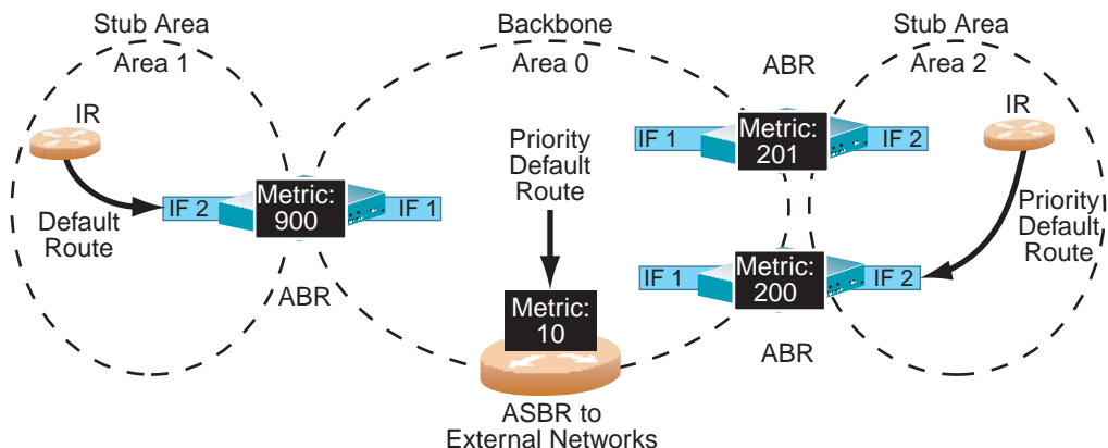
Figure 4-3 Injecting Default Routes
