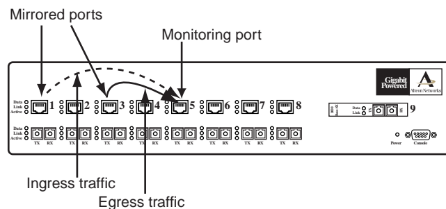
Figure 5-2 Monitoring Ports
