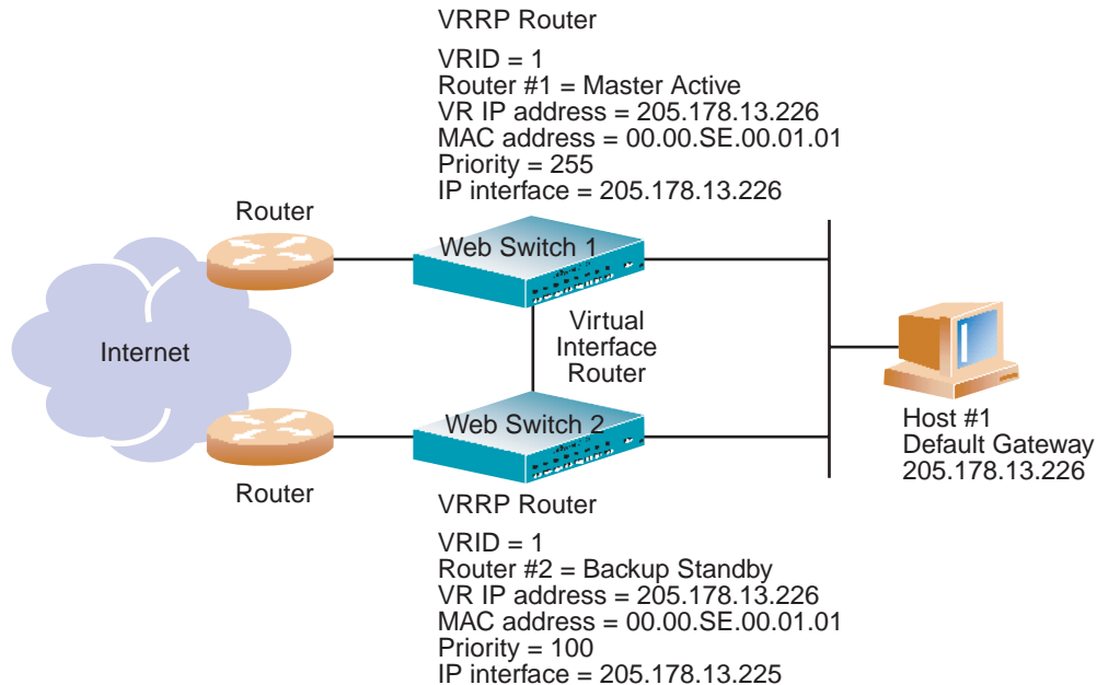
Figure 11-1 Example 1: VRRP Router
