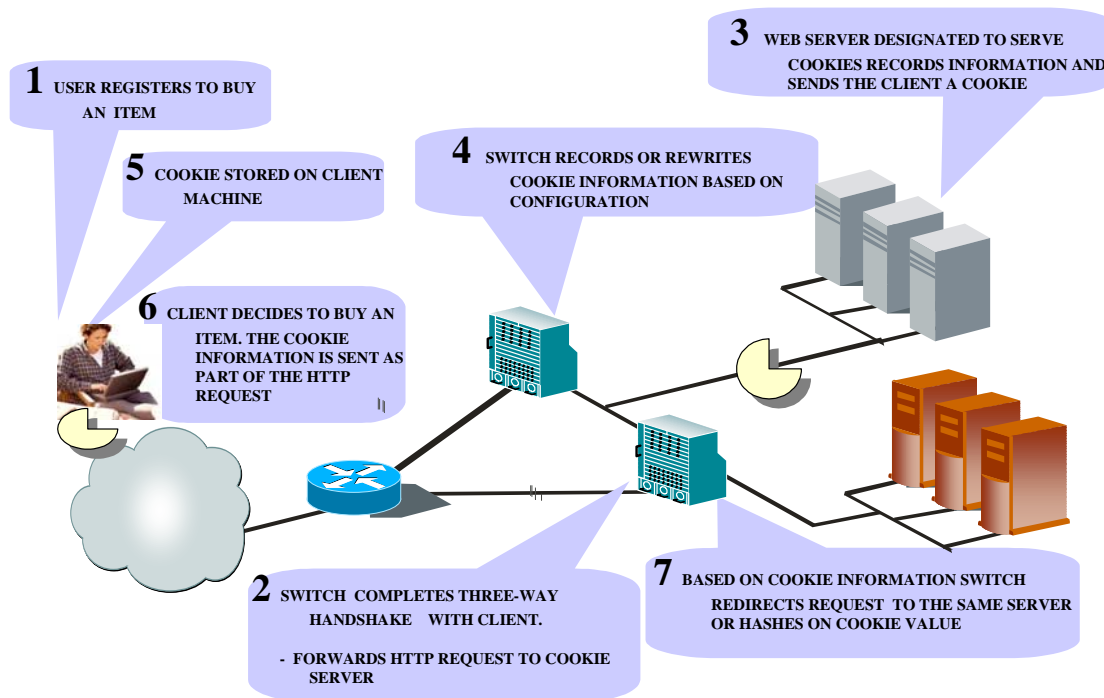
Figure 16-1 Cookie-Based Persistence: How It Works
