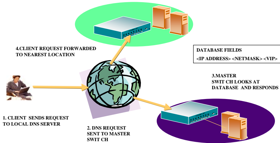
Figure 12-5 GSLB Proximity Tables: How They Work
