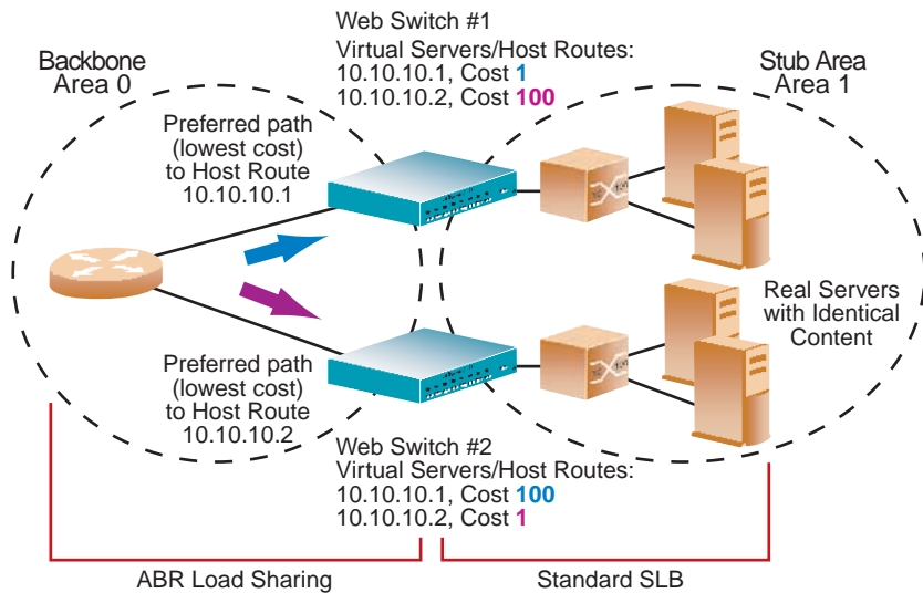
Figure 4-8 Configuring OSPF Host Routes
