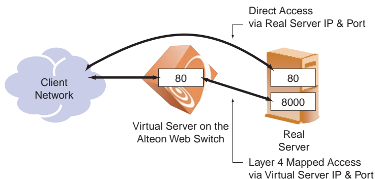
Figure 6-8 Mapped and Nonmapped Server Access
