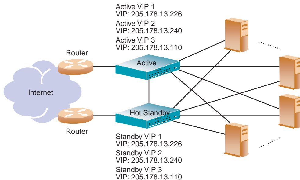
Figure 11-6 Hot-Standby Redundancy
