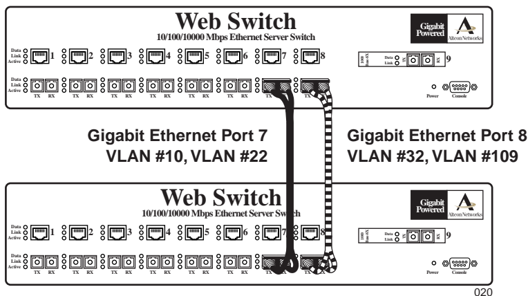
Figure 2-2 Example 2: Parallel Links with VLANs
