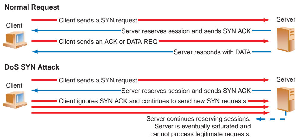
Figure 6-9 DoS SYN Attacks without Delayed Binding
