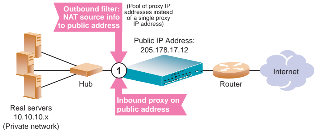
Figure 7-10 Active FTP for Dynamic NAT
