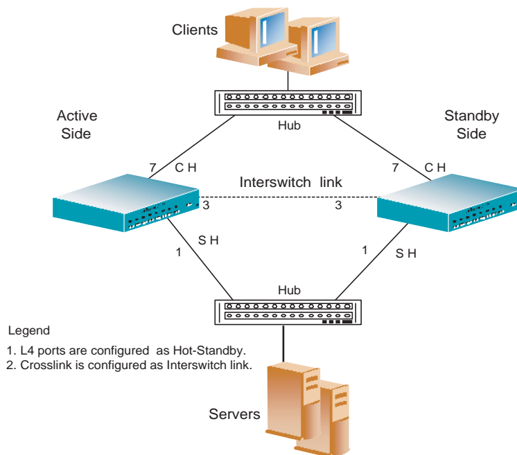
Figure 11-10 Hot-Standby Configuration
