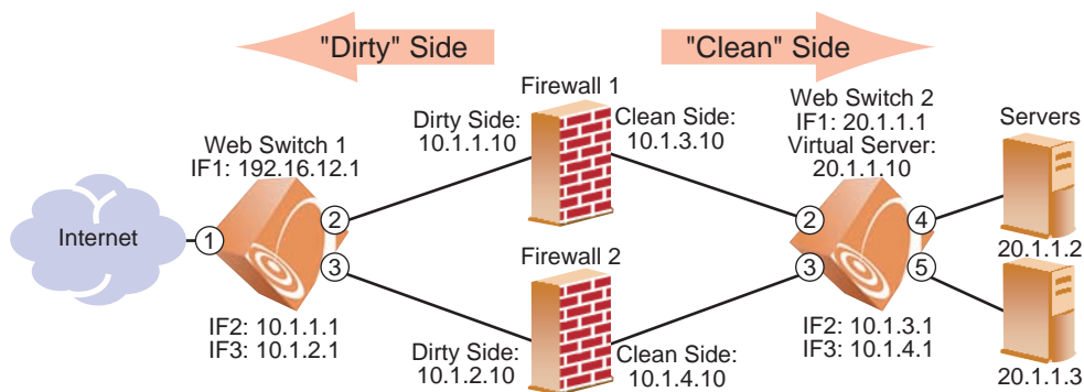
Figure 13-8 Basic FWLB Example Network
