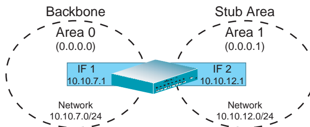
Figure 4-5 A Simple OSPF Domain
