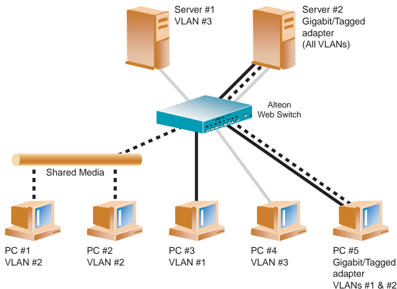
Figure 2-1 Example 1: Multiple VLANs with Tagging Gigabit Adapters
