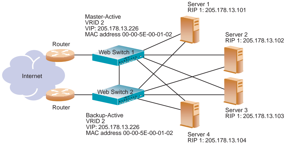
Figure 11-9 Active-Active High-Availability Configuration
