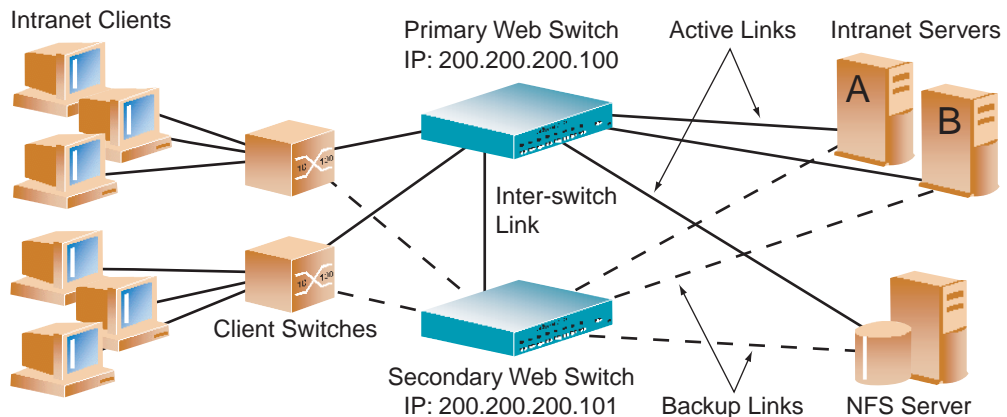
Figure 11-3 A Non-VRRP, Hot-Standby Configuration
