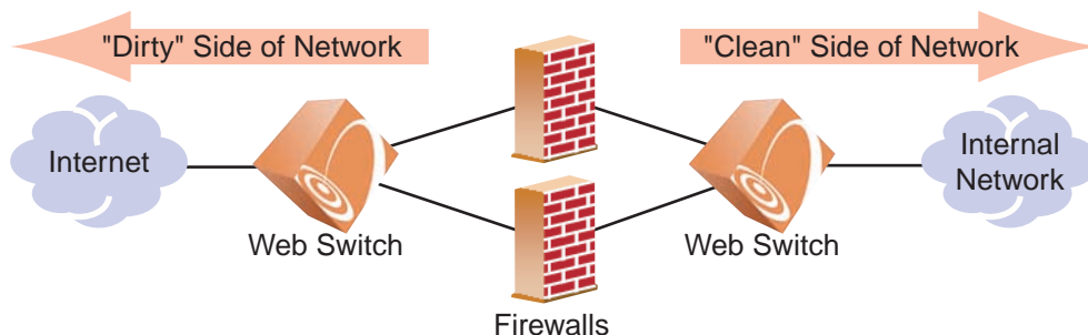
Figure 13-2 Basic FWLB Topology
