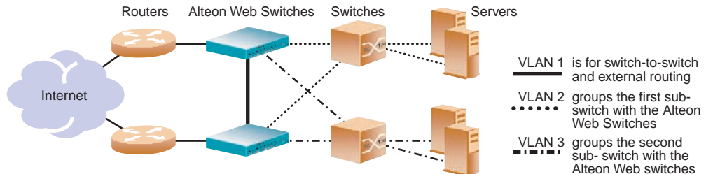
Figure 11-13 Using VLANs to Create Non-Looping Topologies
