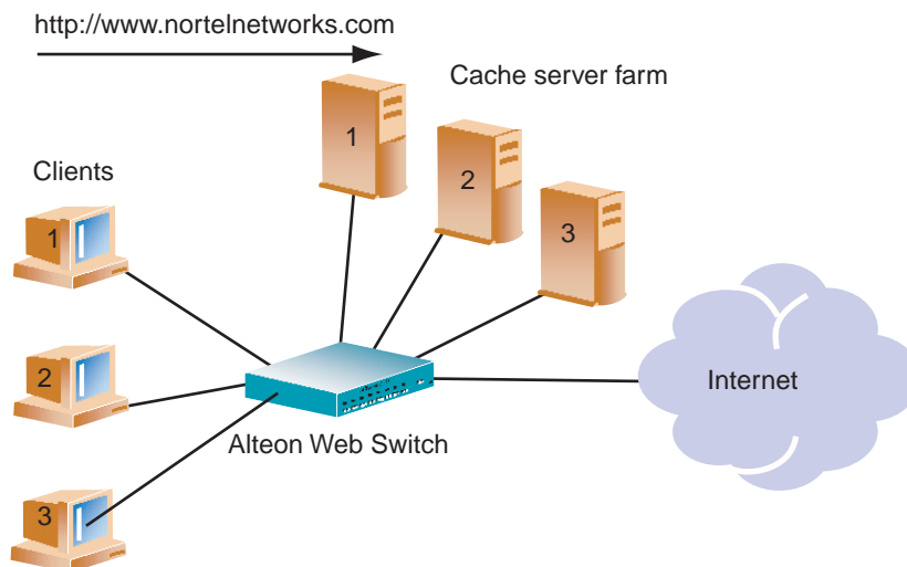
Figure 15-6 URL Hashing for WCR
