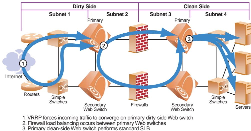
Figure 13-6 Four-Subnet FWLB Process
