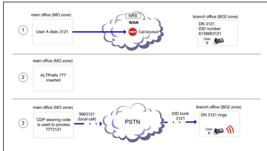
Figure 69 Digits dialed and outpulsed with Alternative Call Routing for NBWM
