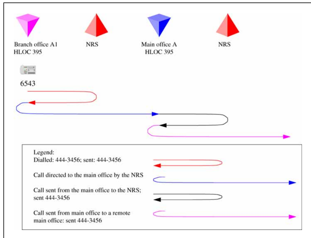
Figure 48 Call to a remote branch office on the originator side
