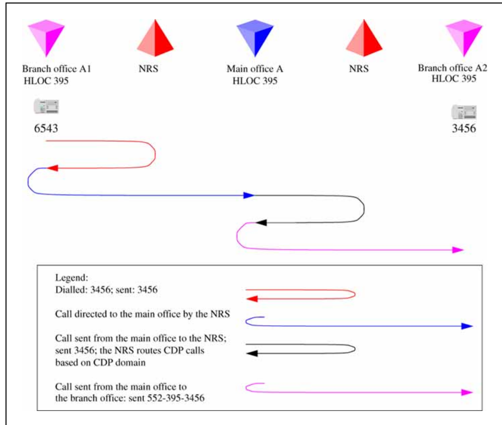
Figure 59 Call flow for Scenario 2 - local call to remote branch office (originator side)
