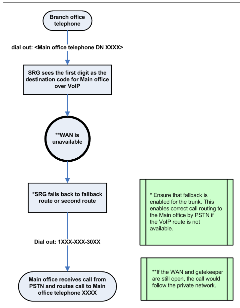
Figure 16 Local Mode: SRG telephone calls a main office telephone
