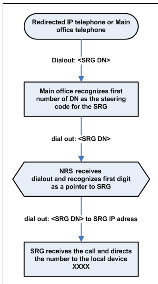
Figure 13 Normal Mode: Main office telephone calls an analog phone at the SRG
