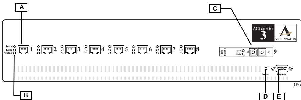
Figure 3 Alteon AD3 Front Panel
