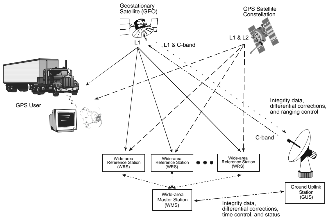
Figure 2-1 The WAAS Concept
