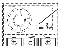
Button Frequency Jumpers (inside pushbutton case)
