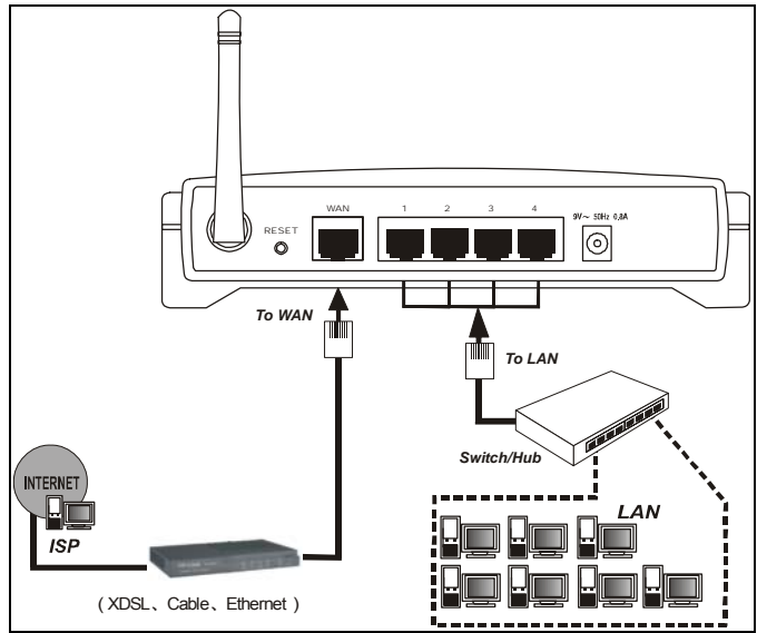
Figure 3-1: Hardware Installation of the RW400SG 108Mbps Wireless Router
