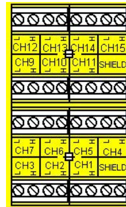
Thermocouple Channel Connections for DaqTemp14 and DaqTemp14A
