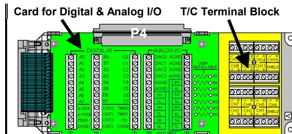
DaqTemp14 and DaqTemp14A Modules, Internal Layout*
