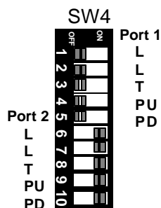
Figure 1: Switch SW4
