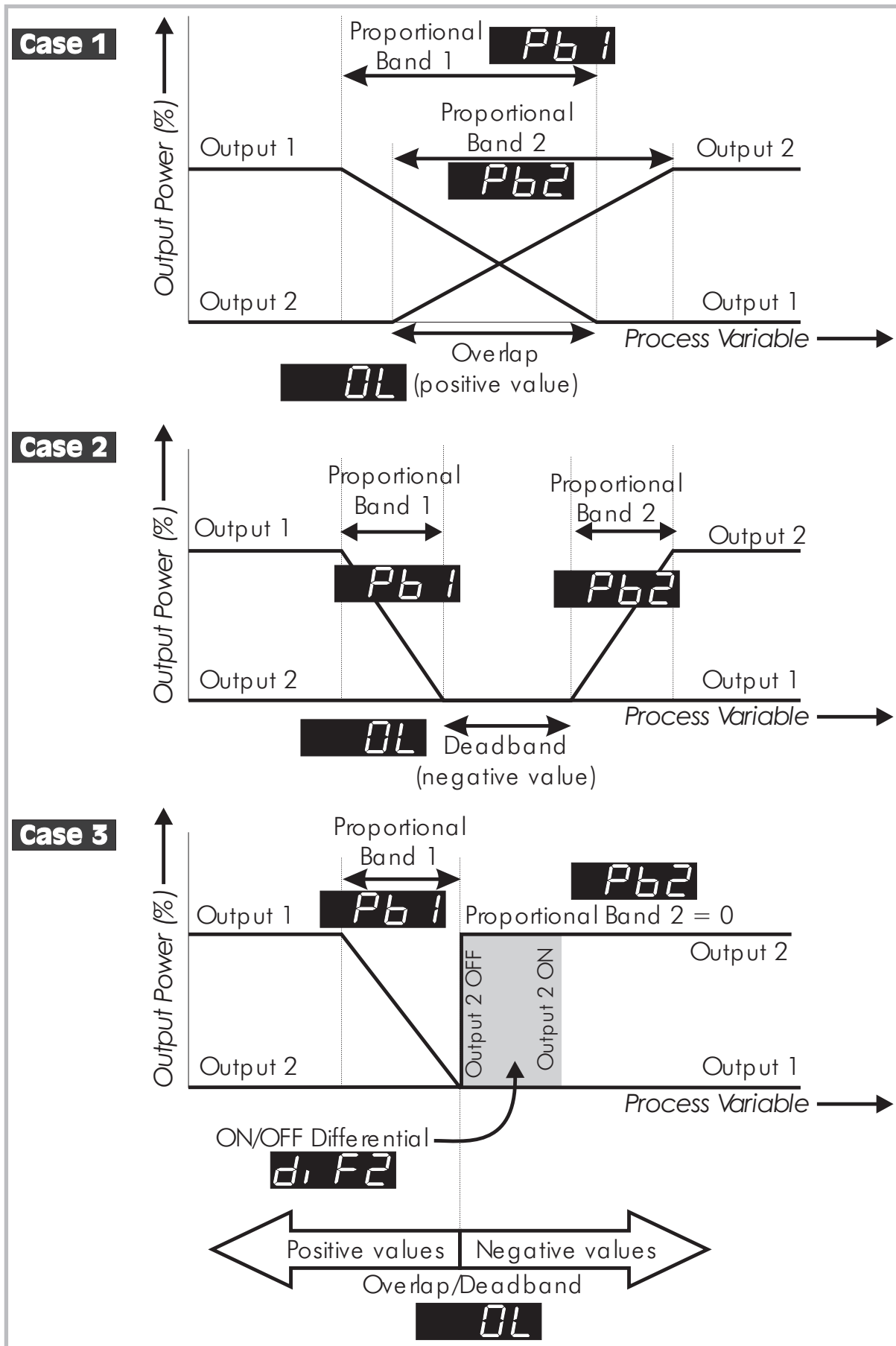
Figure 2-1 Proportional Band and Overlap/Deadband
