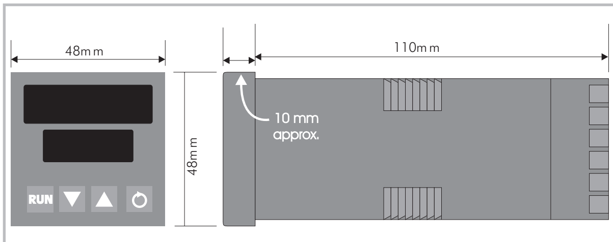
Figure 1-2 Main Dimensions
