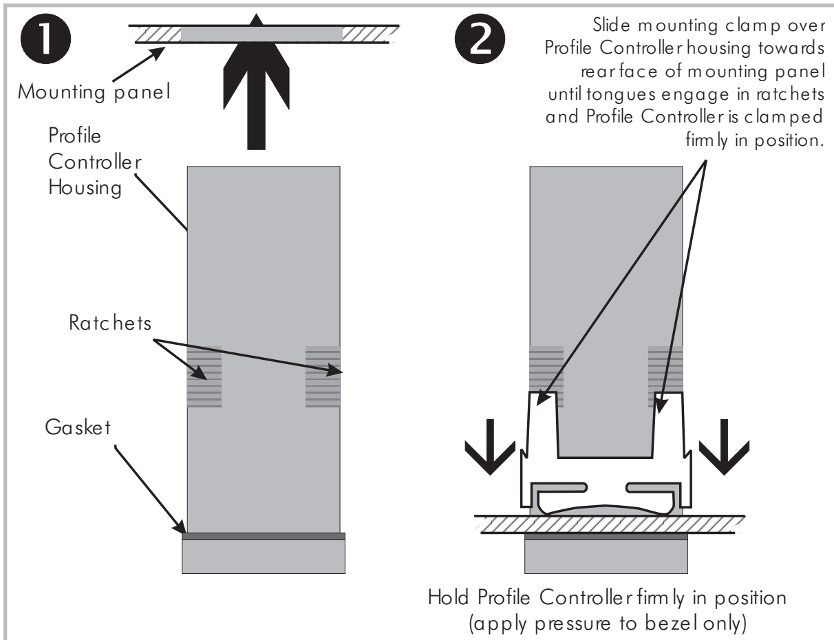
Figure 1-3 Panel-Mounting the Profile Controller
