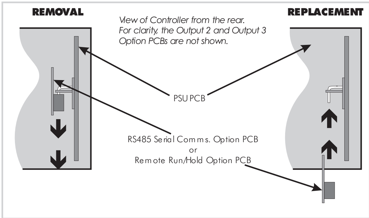
Figure 2-3 Removing the RS485 Communications Option PCB or the Remote Run/Hold Option PCB
