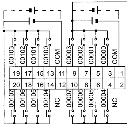
Input Connector
