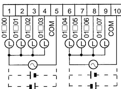
Terminal Block #1 (Left side)
