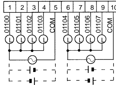
Terminal Block #2 (Right side)
