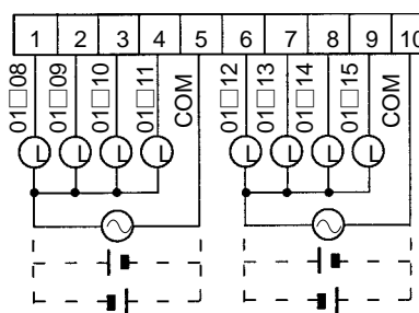
Terminal Block #2 (Right side)
