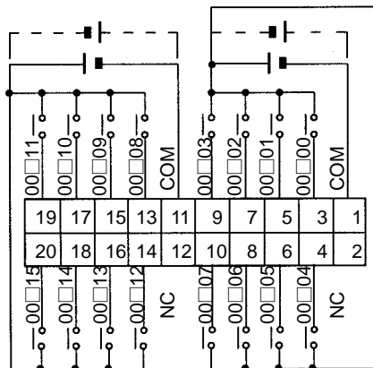
Input Connector
