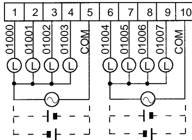
Terminal Block #1 (Left side)
