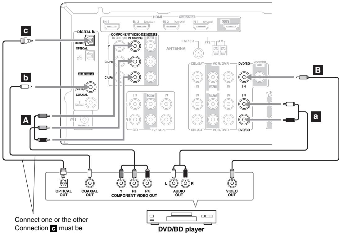
DVD/BD player
