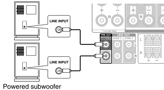
Powered subwoofer
