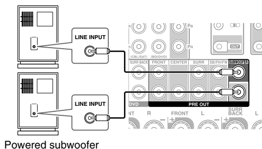
Powered subwoofer
