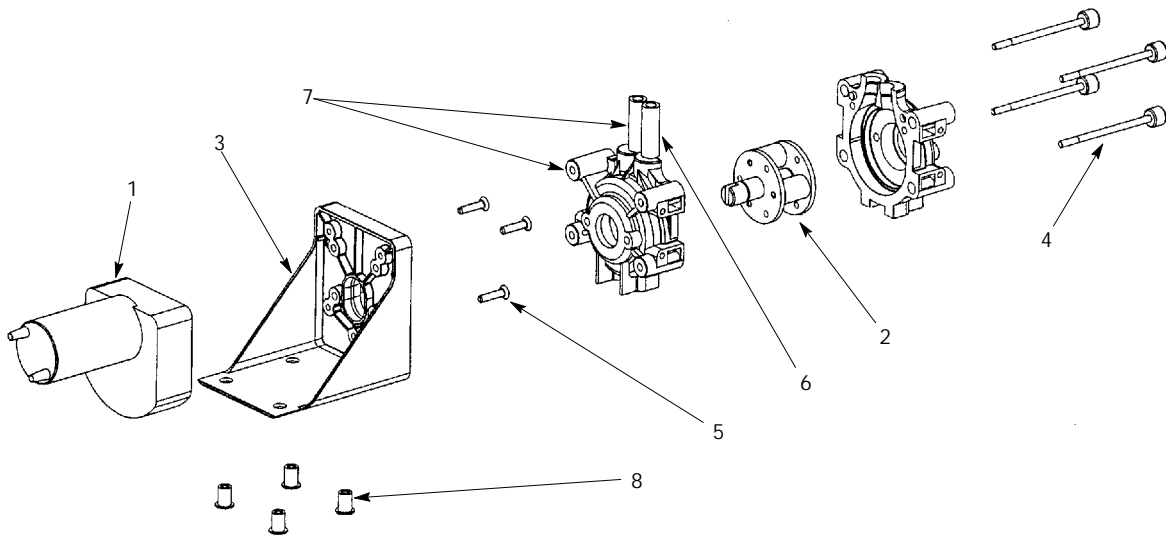
FIGURE 5. PUMP MOTOR ASSEMBLY
