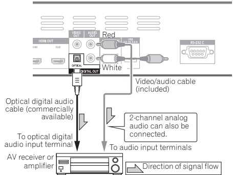
BDP-LX55's rear panel
