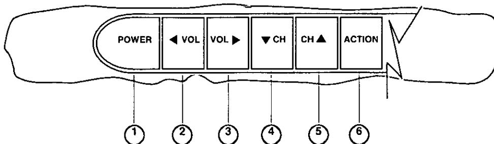
Front Panel for CT-2520H Panel frontal para CT-2520H
