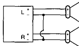
INCORRECT Speaker Common (common earth lead)
