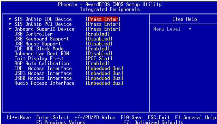
Figure 3.4: Integrated peripherals
