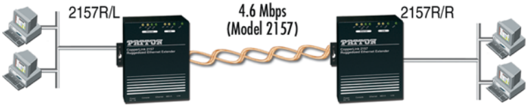
Figure 1. Typical application
