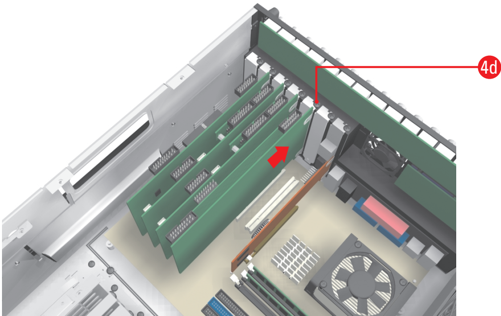
Figure 12. Securing the DX8000-MUX16 Card
