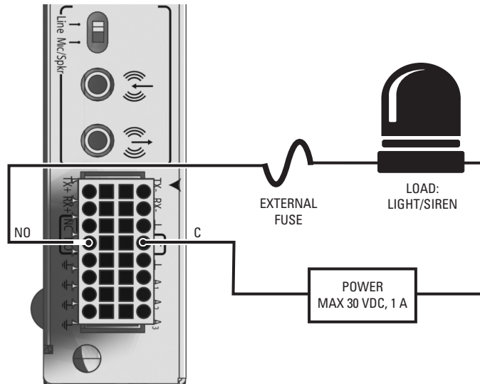
Figure 13. Connecting a Relay Device
