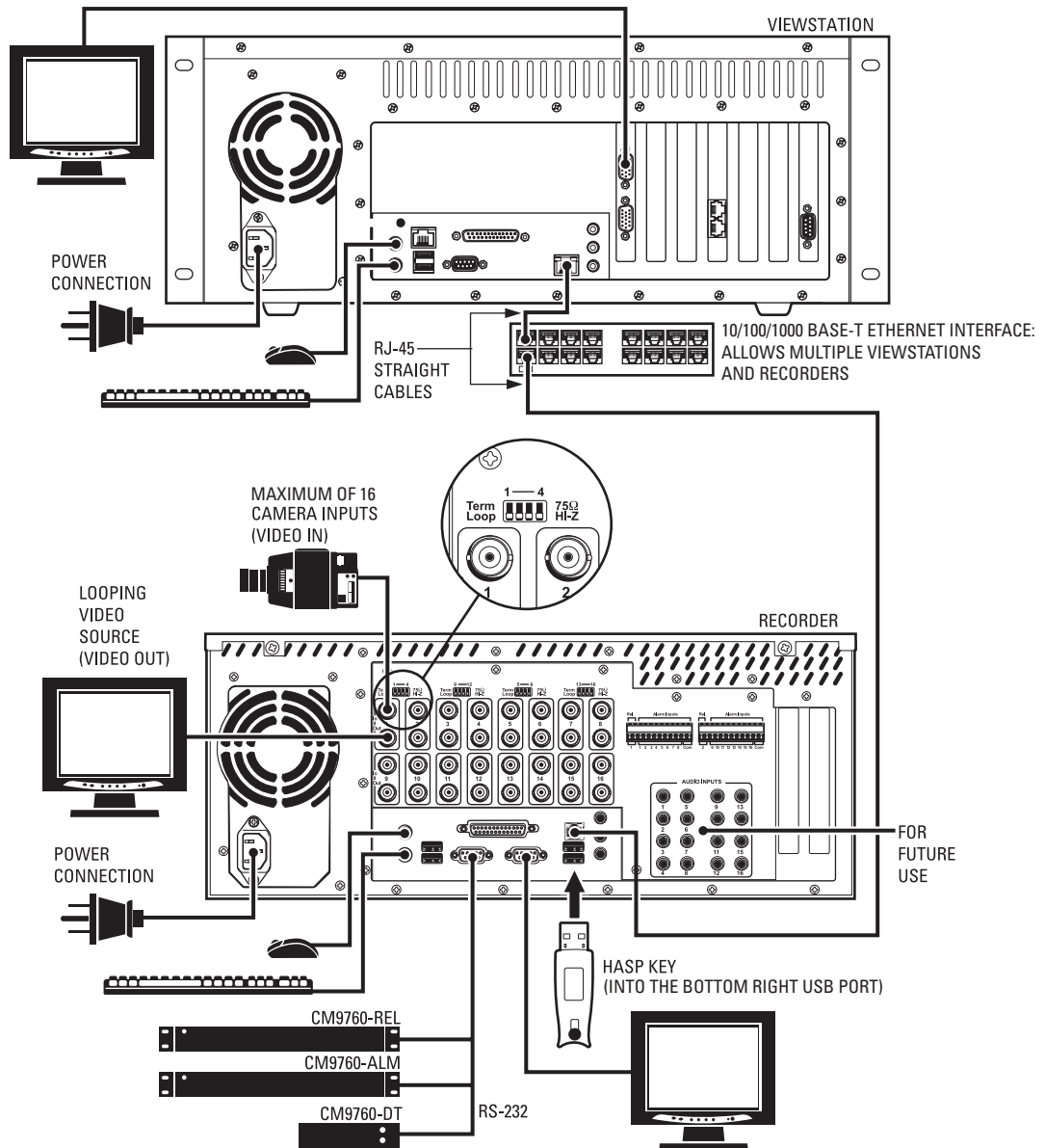
Figure 8. System Connections
