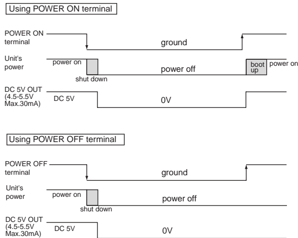
Figure 8. Operation of Power On and Power Off Terminals
