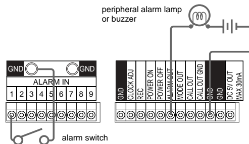
Figure 6. Alarm Input and Output Connections
