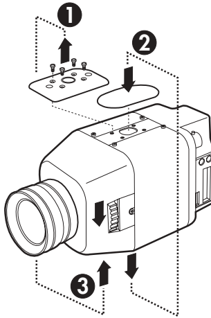
Figure 3. Camera Mounting
