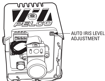
FIXED LENS
