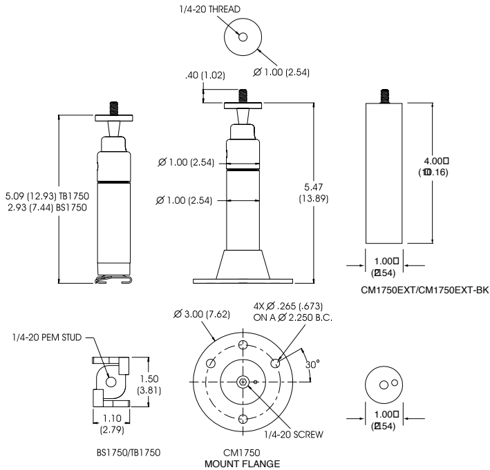
Figure 2. CM1750EXT/CM1750EXT-BK and BS1750/CM1750/CM1750-BK/TB1750 Dimension Drawing
