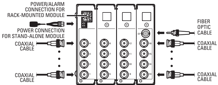
Figure 5. FT8316 Transmitter/FR8316 Receiver Connections
