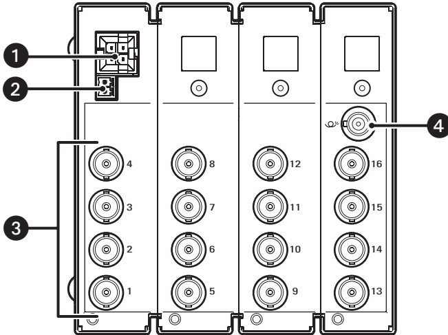
Figure 4. Rear Panel of FT8316 Transmitter and FR8316 Receiver
