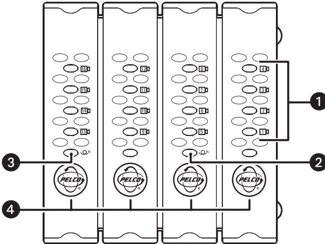
Figure 2. Front Panel of FT8316 Transmitter
