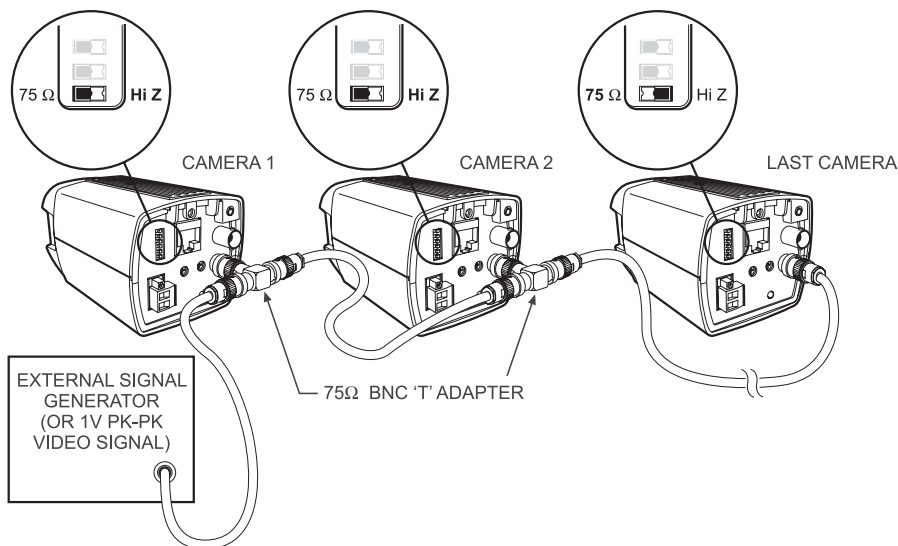
Figure 4. Genlock Daisy-chain Connection
