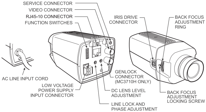
Figure 1. Camera Layout
