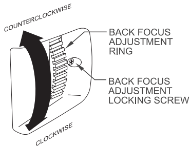
Figure 8. Back Focus Adjustment
