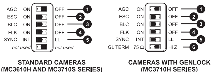
Figure 9. Switch Settings (White indicates default switch position.)
