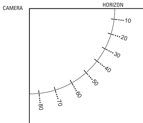
Figure 3. Window Blank Tilt Angles
