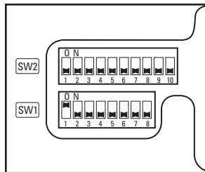
Figure 1. Default Switch Settings
