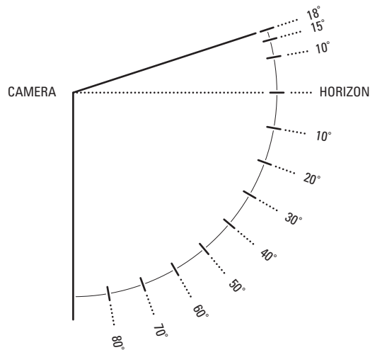
Figure 7. Window Blank Tilt Angles
