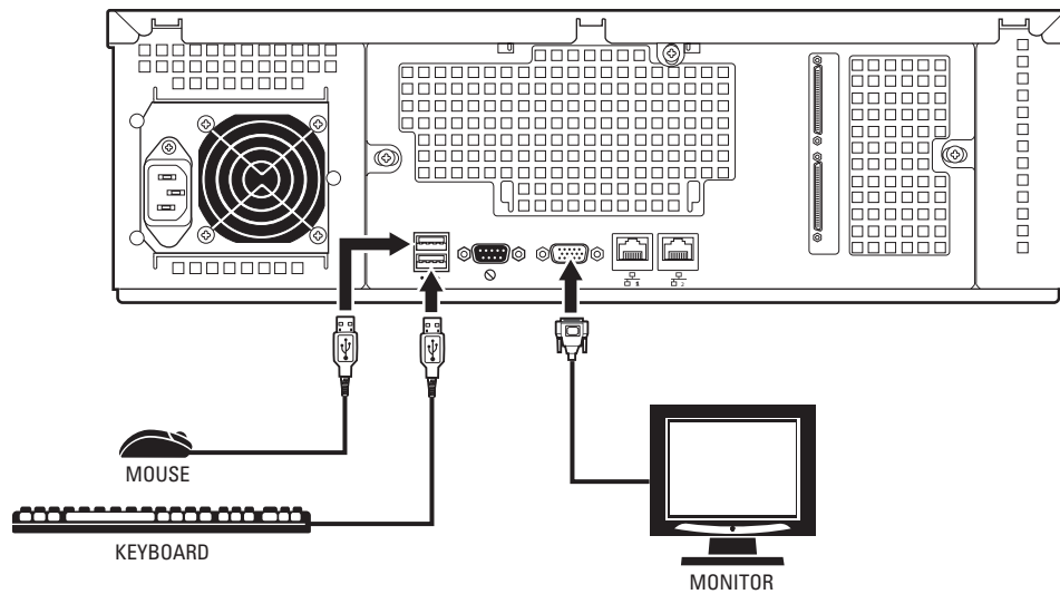
Figure 6. Keyboard, Mouse, and Monitor Connections
