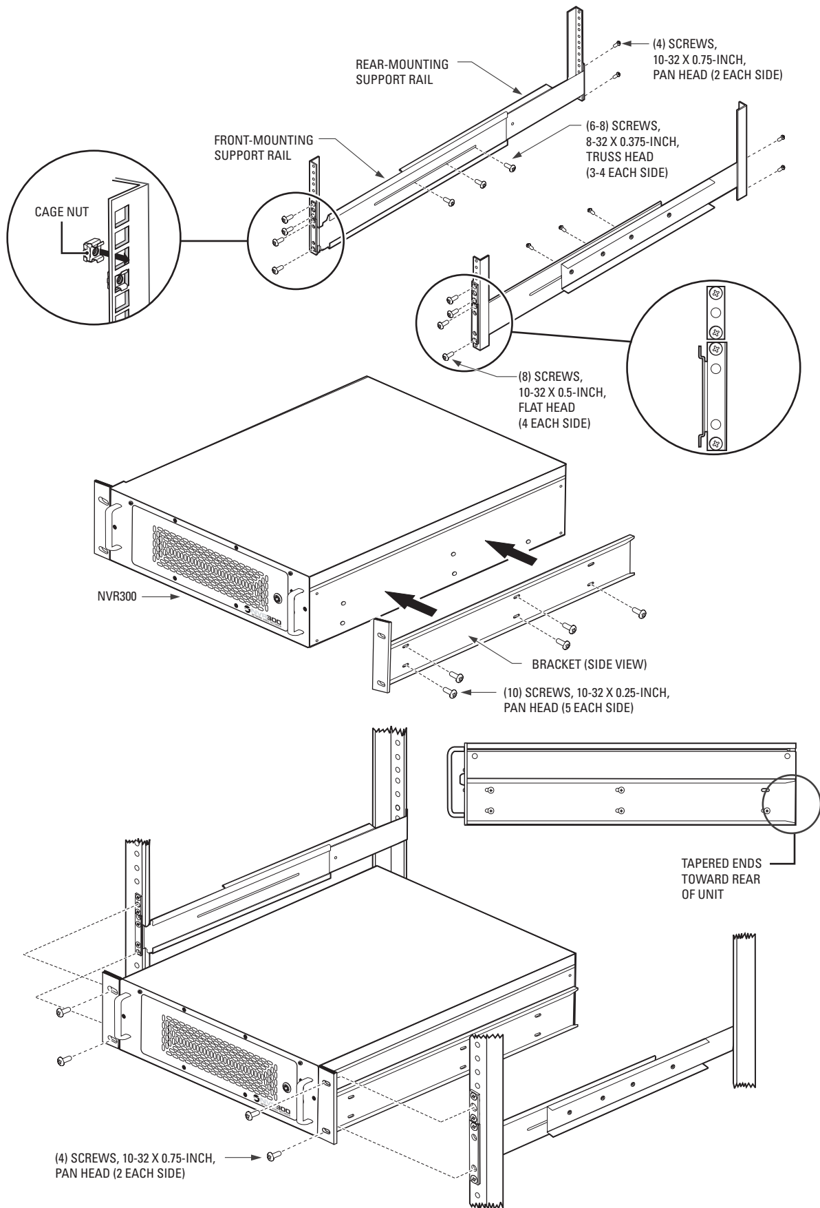
Figure 4. NVR300 Rack-Mount Installation
