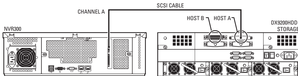
Figure 44. NVR300 Connection to One DX9200HDDI Video Storage Unit
