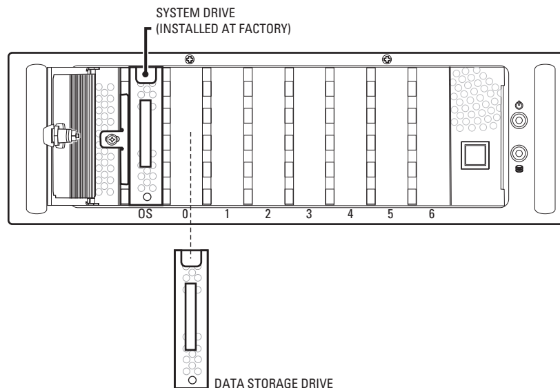
Figure 5. Hard Disk Drive Installation
