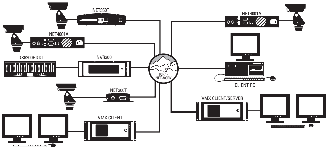
Figure 1. Sample NVR300 Application
