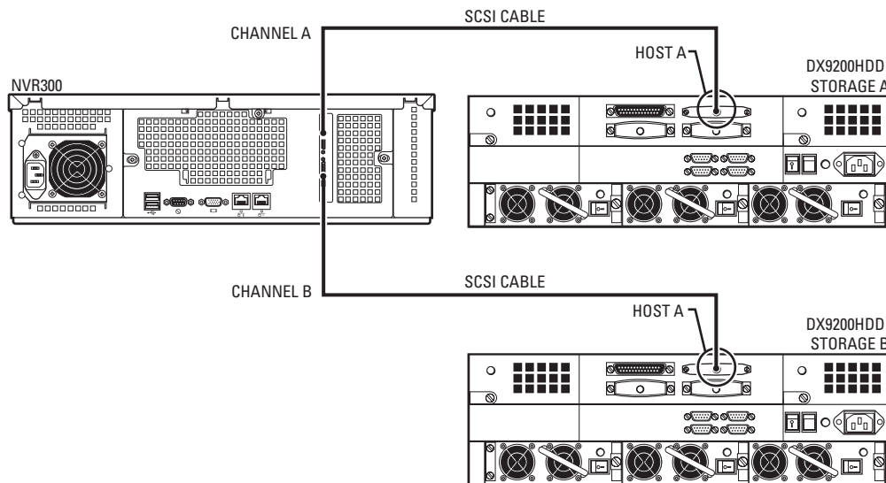
Figure 45. NVR300 Connection to Two DX9200HDDI Video Storage Units
