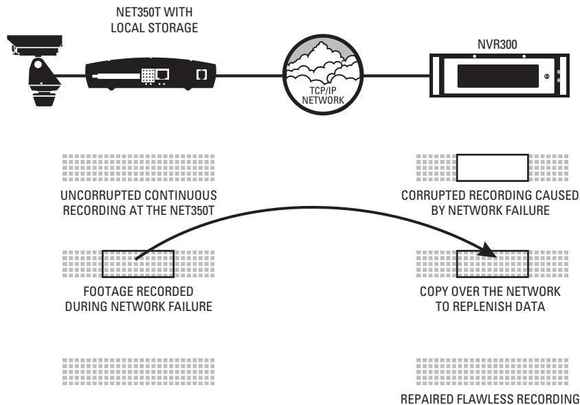
Figure 47. Automatic Data Replenishment at NVR300
