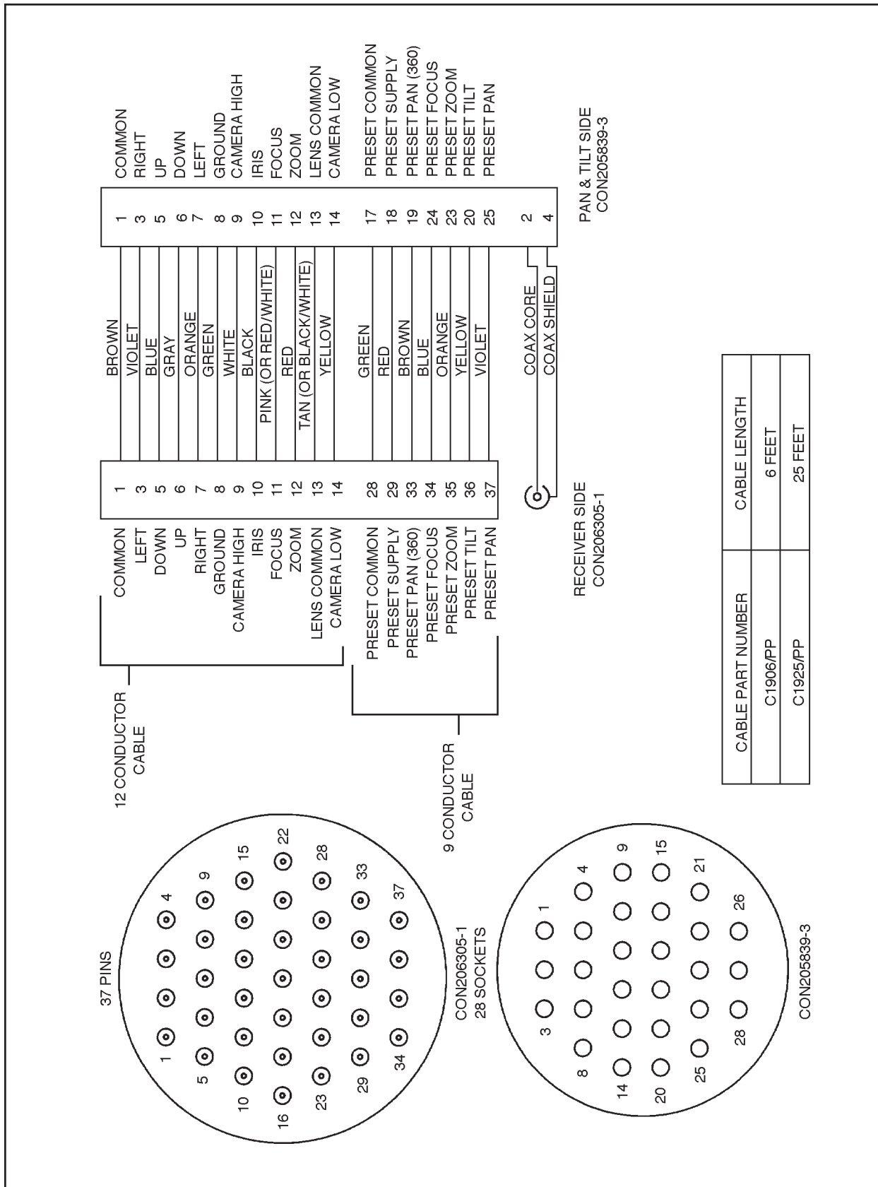
Figure 3. C1906/PP and C1925/PP Wiring Diagram for Use with Upright Pan/Tilts Only
