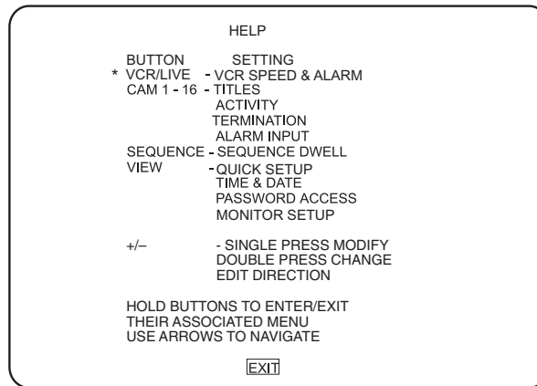
Figure 10. Help Menu
