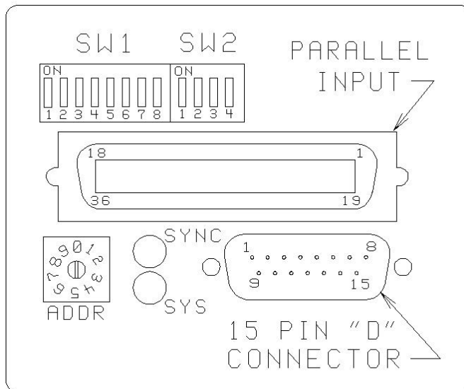
CX/TX Interface.
